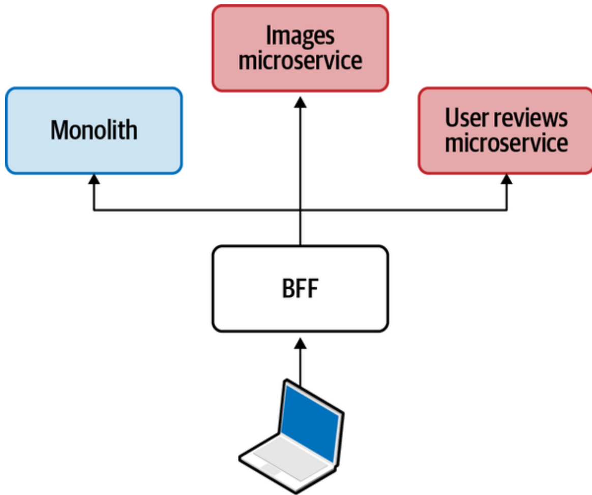
Figure 8-13. The microservices boxes represent services extracted from the monolith and converted to microservices. The BFF layer allows the client to be unaware of the change happening in the backend, maintaining the same contract at the BFF level.
