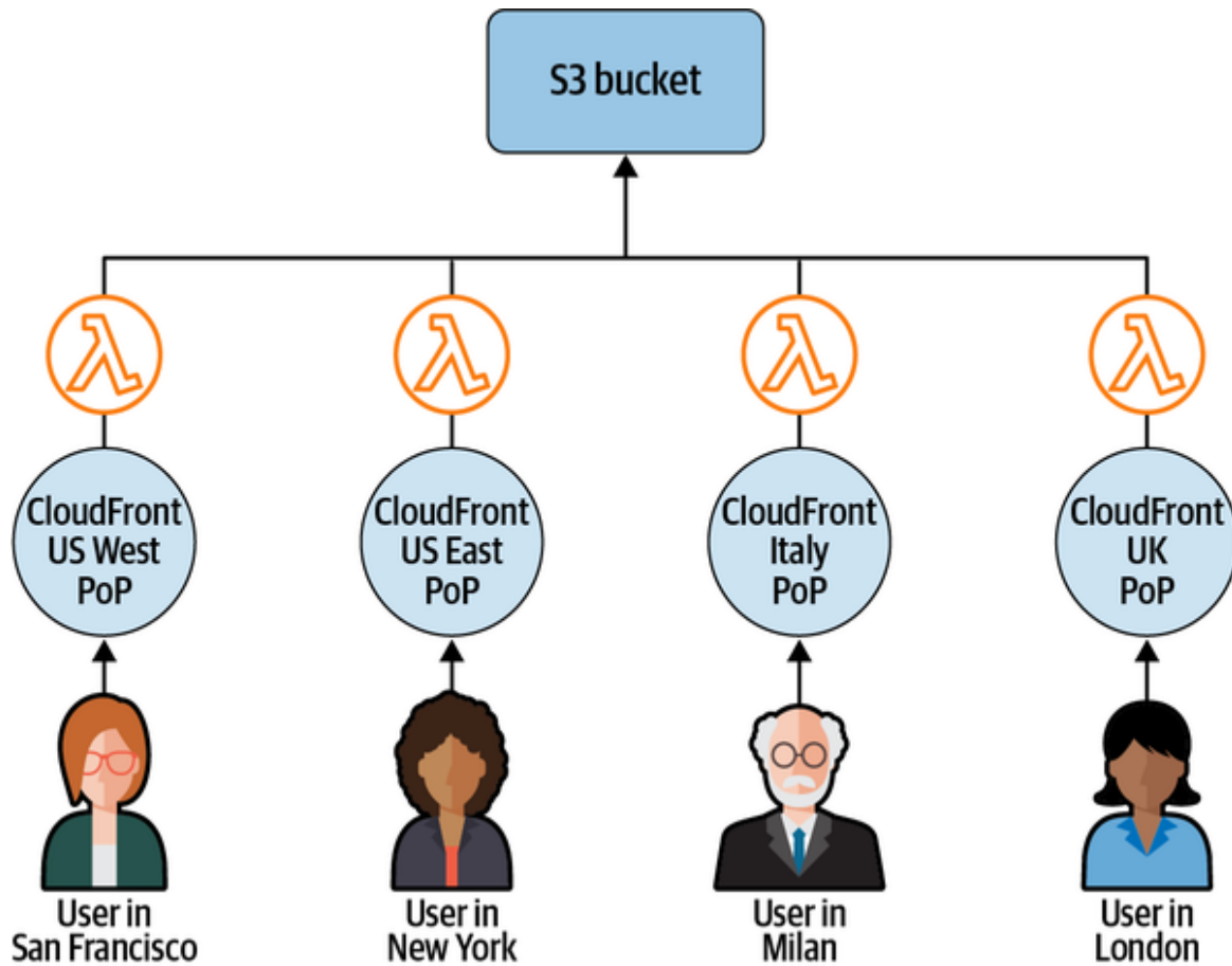
Figure 9-10. Simple infrastructure based on S3 bucket, Lambda@Edge, and a CDN like Amazon CloudFront distribution, with point of presence (PoP) available all over the world
