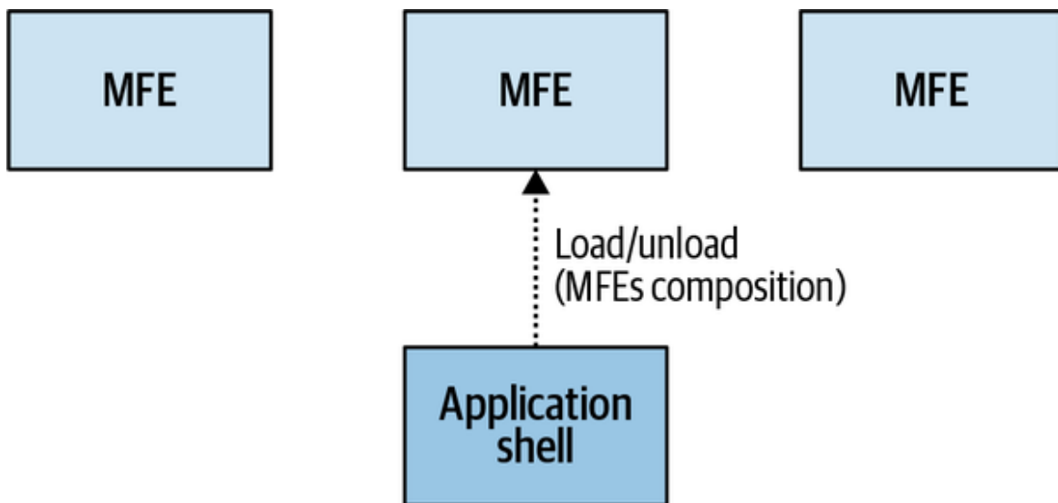
Figure 9-6. Client-side composition, where the application shell is responsible for loading and unloading one micro-frontend at a time
