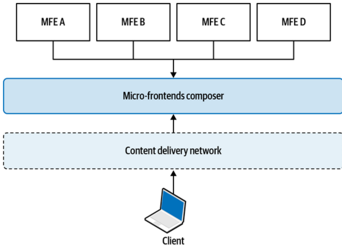
Figure 4-23. A typical high-level architecture for a server-side micro-frontend architecture, where a composer is responsible for stitching together the different micro-frontends at runtime. A CDN can be used for offloading traffic to the origin.
