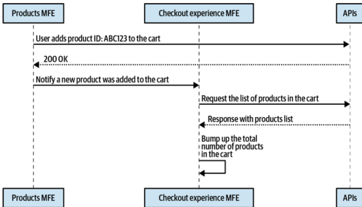
Figure 4-24. An example of how the product's micro-frontend notifies the checkout experience micro-frontend to refresh the cart interface when a user adds a product to the cart
