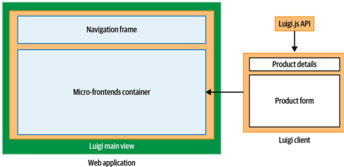
Figure 4-22. A micro-frontend architecture (at left) with the Luigi framework is composed of two parts: the main view and a Luigi client. The Luigi.js API provides an abstraction for common operations, such as communication between a micro-frontend and the host.
