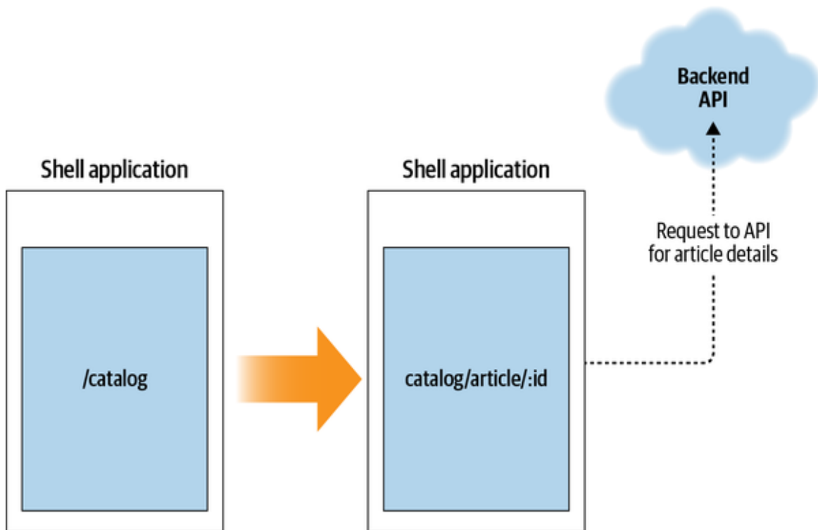
Figure 3-7. Micro-frontends communication via query strings or URL
