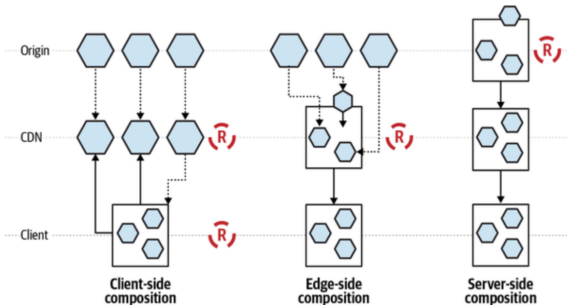
Figure 3-4. Micro-frontends routing diagram
