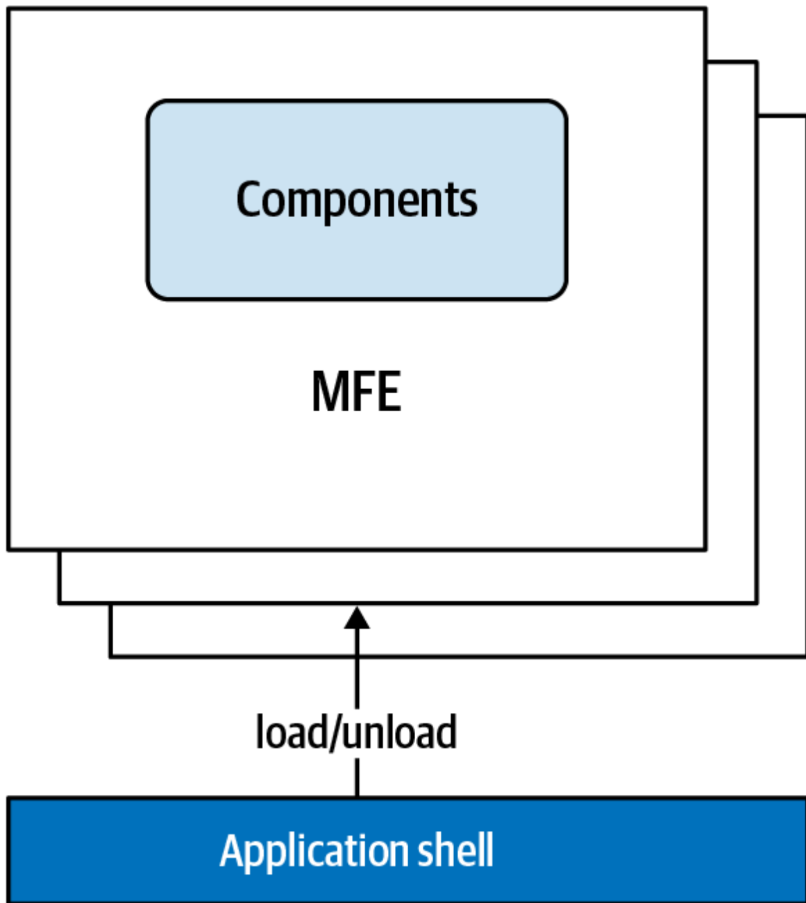
Figure 4-4. Vertical-split architecture with client-side composition and routing using the application shell
