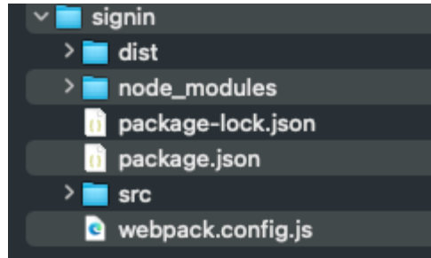
Figure 5-4. Micro-frontend structure
