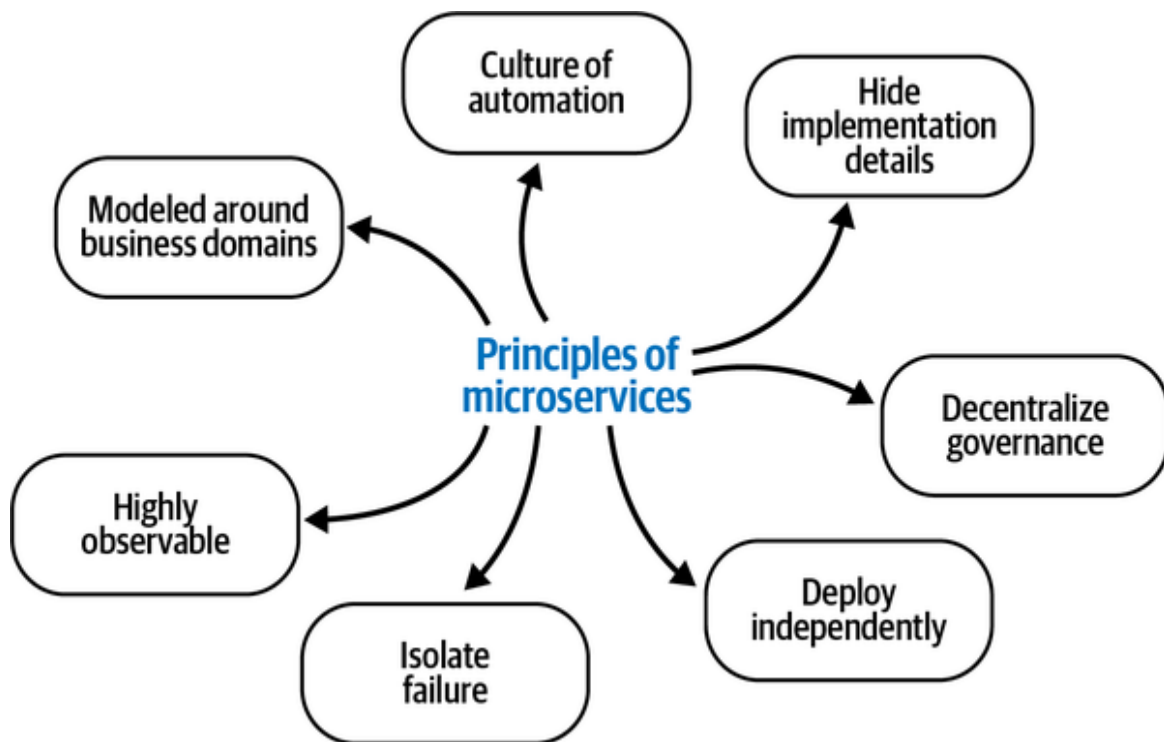
Figure 2-4. Microservices principles
