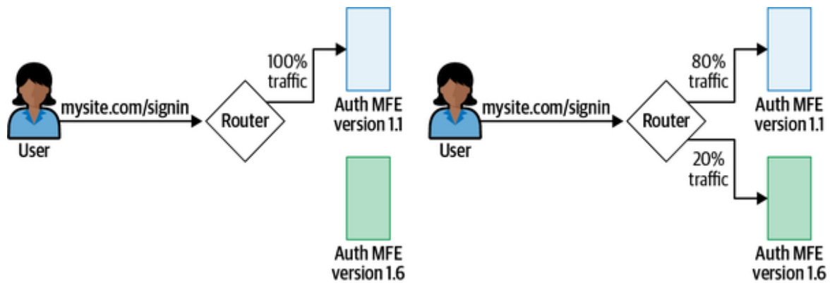
Figure 6-7. Canary release
