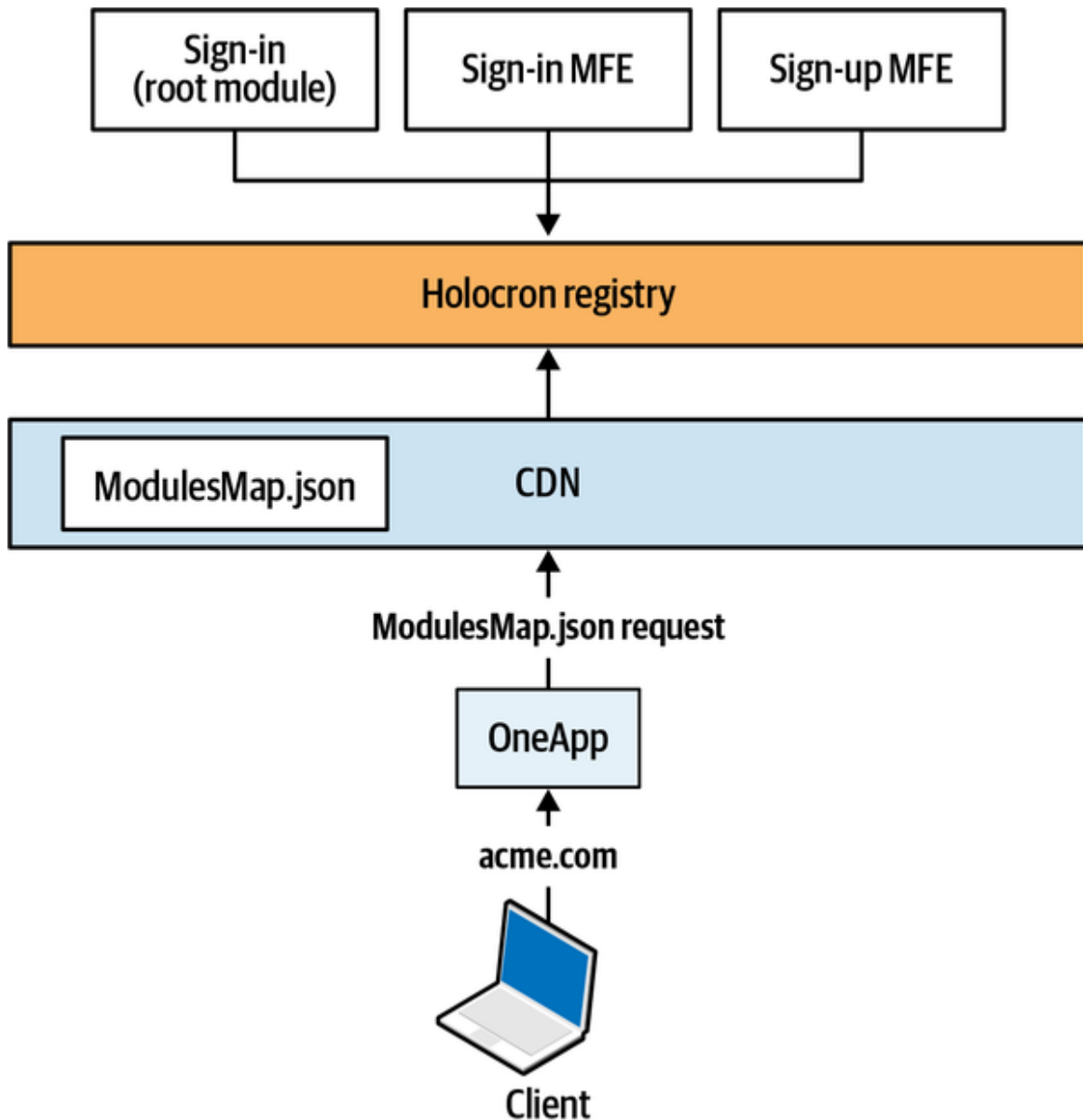
Figure 4-25. Holocron is a server-side rendering system for micro-frontends
