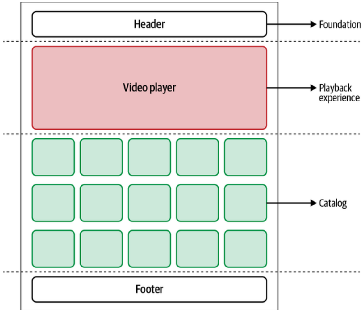
Figure 4-12. The catalog view is composed by the application shell, which loads two micro-frontends: the playback experience and the catalog itself
