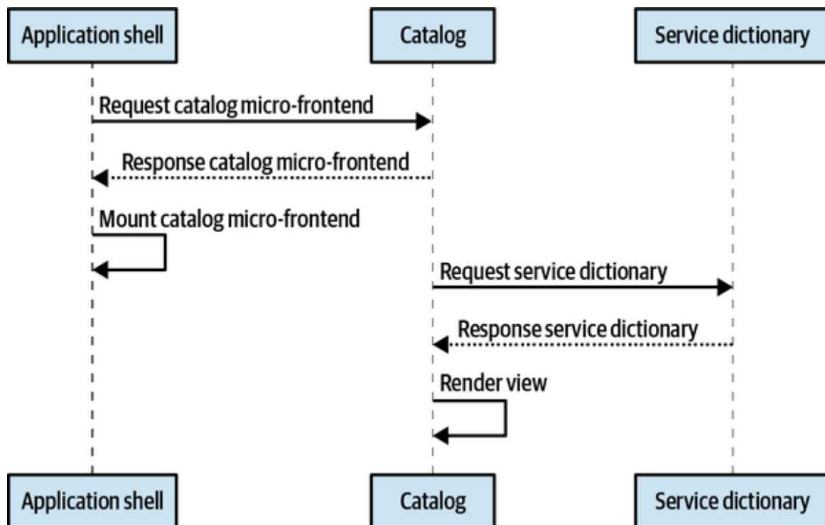
Figure 8-4. Sequence diagram to implement a service dictionary with a vertical-split architecture
