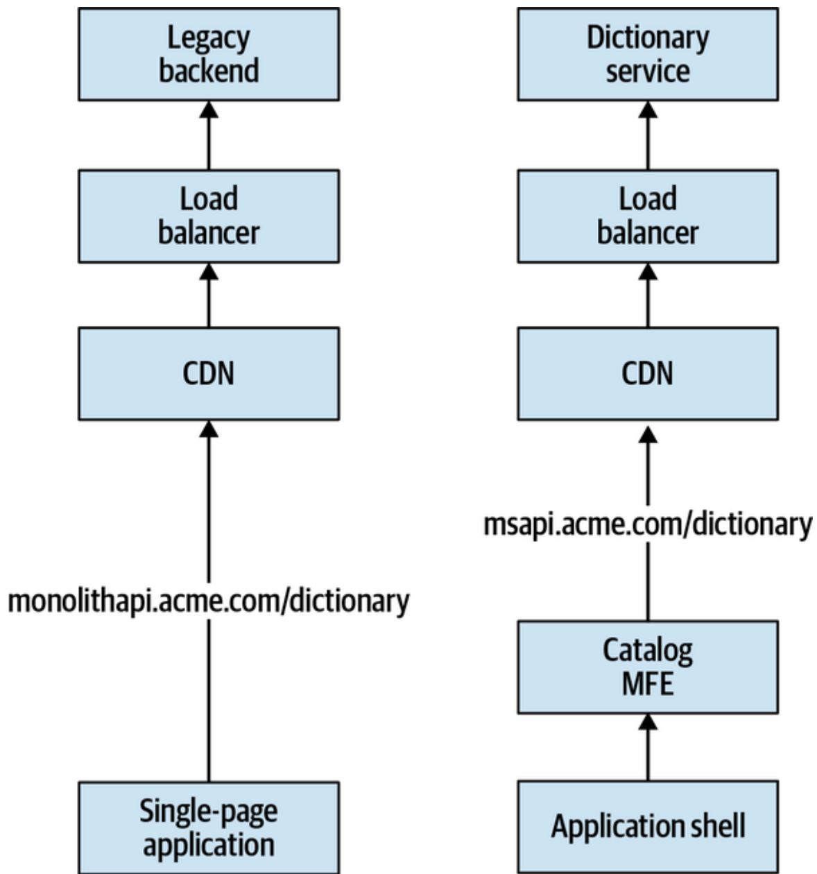
Figure 9-17. The micro-frontend consumes a new API for fetching the labels to display in the interface through a new microservice. The SPA will consume the API from the legacy backend.
