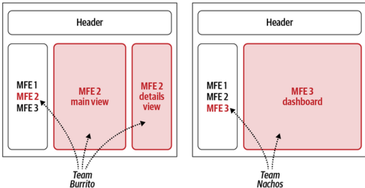
Figure 4-19. New Relic micro-frontend implementation. Every team is responsible for their own domain, and when a user selects a dashboard, the related micro-frontend is lazy-loaded inside the application shell.
