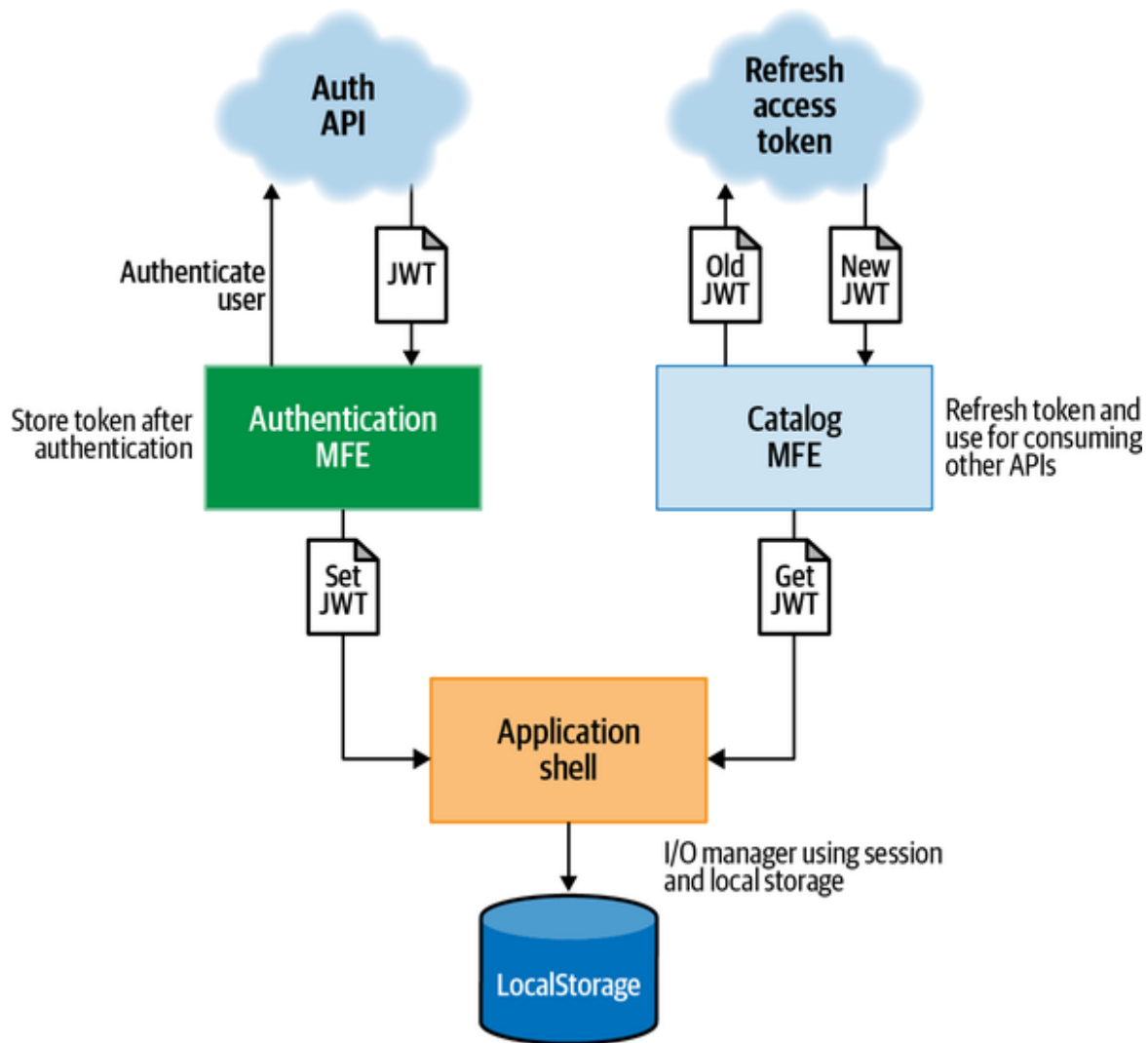
Figure 9-13. When the frontend platform is fully migrated to micro-frontends, every micro-frontend will be responsible for managing part of the users' authentication
