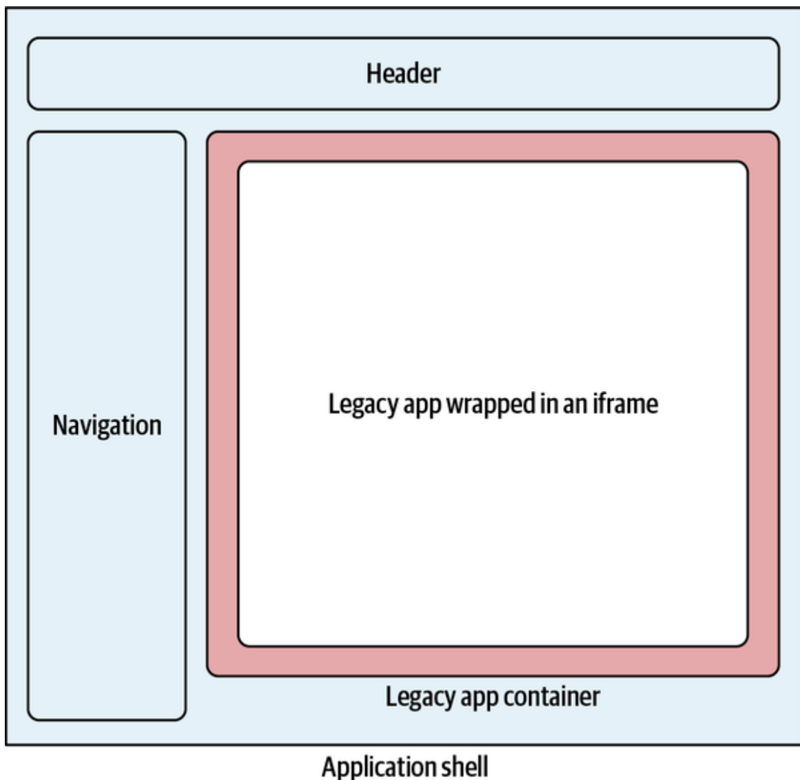
Figure 5-6. The application shell loads a micro-frontend that acts as an adapter between the new and old worlds. The legacy application is wrapped in an iframe to minimize the impact with the existing micro-frontend codebase.
