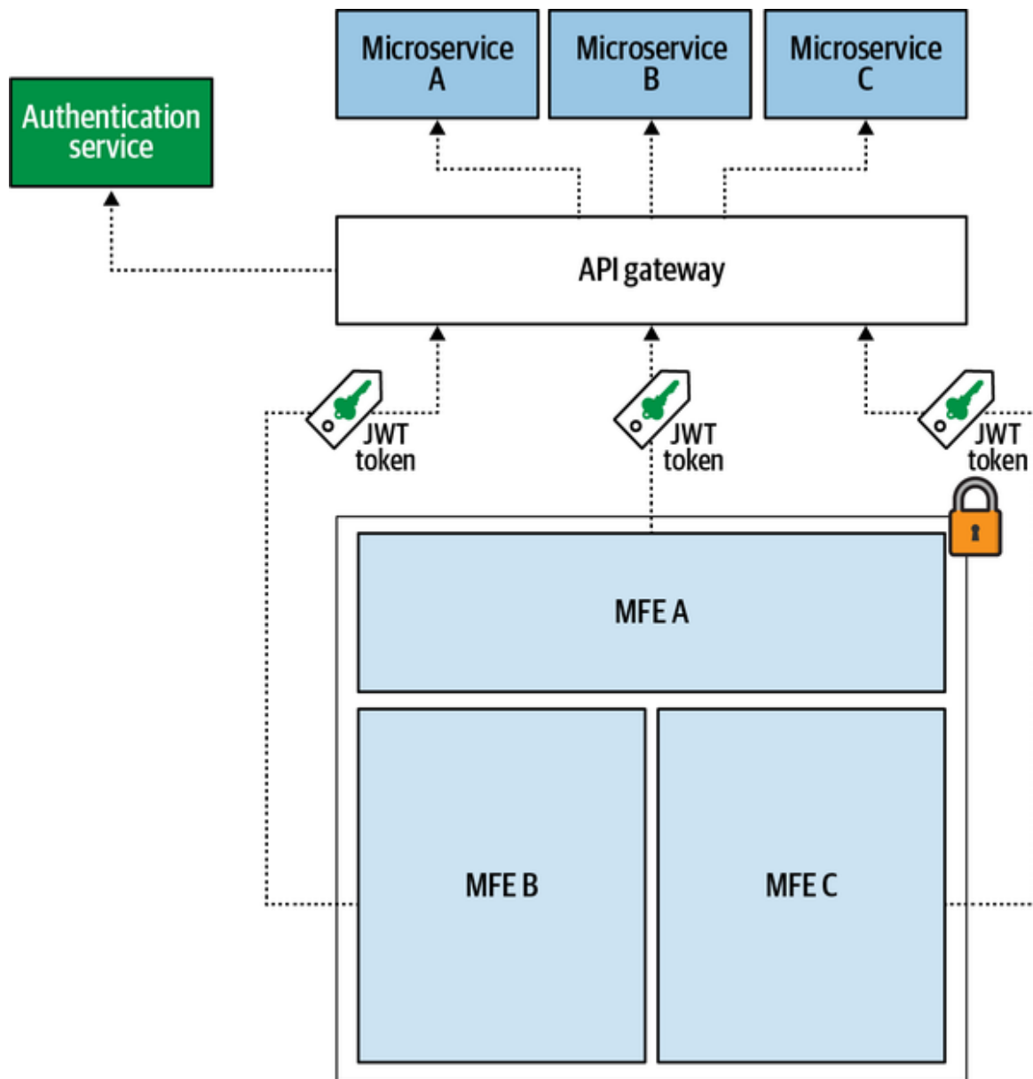
Figure 4-18. Every micro-frontend in a horizontal-split architecture has to fetch data from an API passing a JWT token to the backend to validate that the user is entitled to retrieve the data requested
