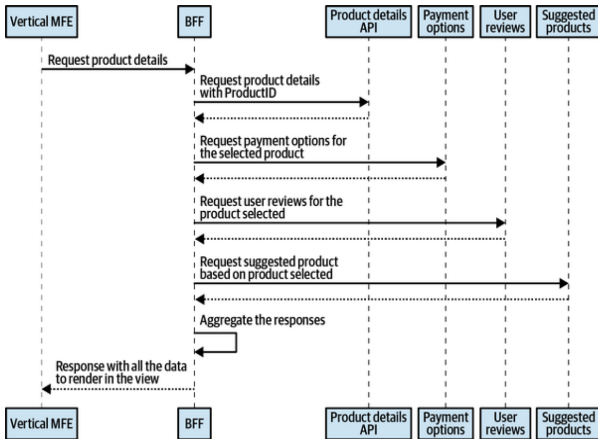
Figure 8-16. Sequence diagram showing the benefits of the BFF pattern used in combination with a vertical split composed on the client side
