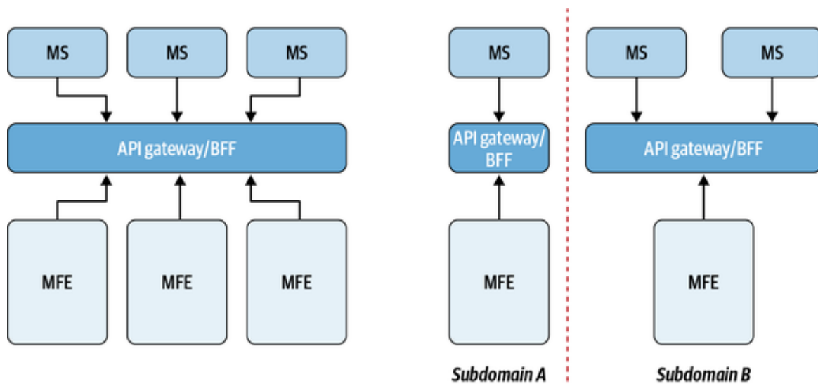
Figure 8-8. On the left is a unique entry point for the API layer; on the right are multiple entry points, one per subdomain
