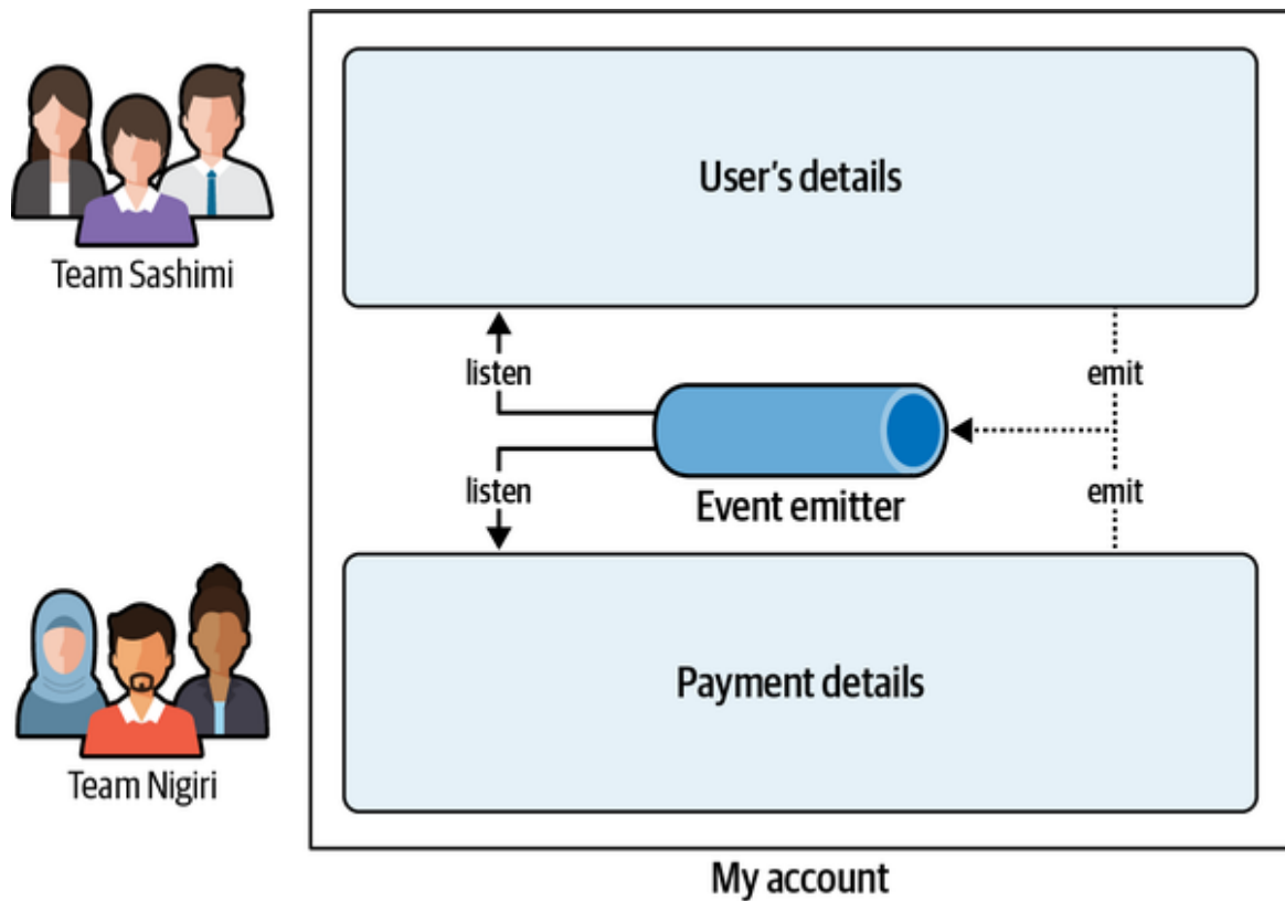
Figure 5-5. Teams Sashimi and Nigiri are implementing an event emitter shared between micro-frontends for communicating the domain's boundaries
