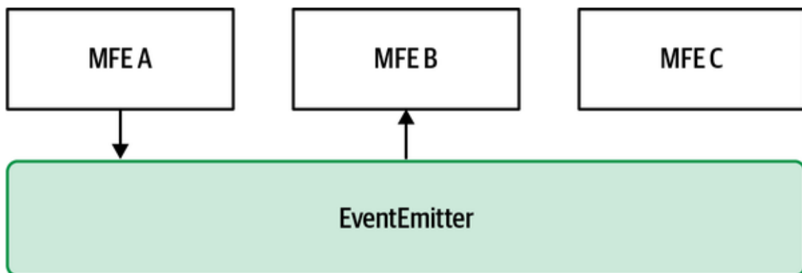
Figure 4-16. MFE A emits an event using the EventEmitter as a communication bus; all the micro-frontends interested in that event will listen and react accordingly
