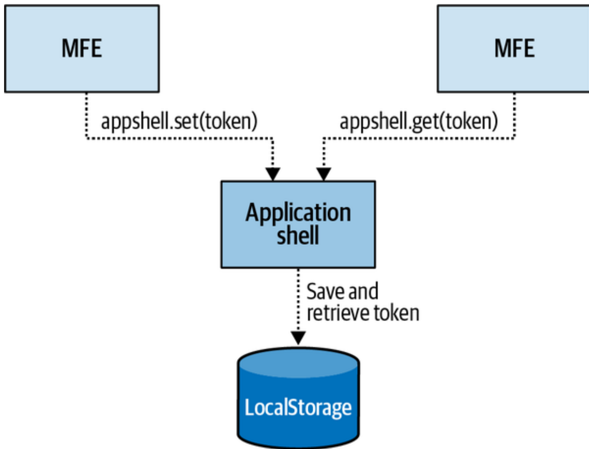
Figure 9-8. The application shell is responsible for storing data in the local storage and exposing several APIs to the micro-frontends for storing and retrieving data
