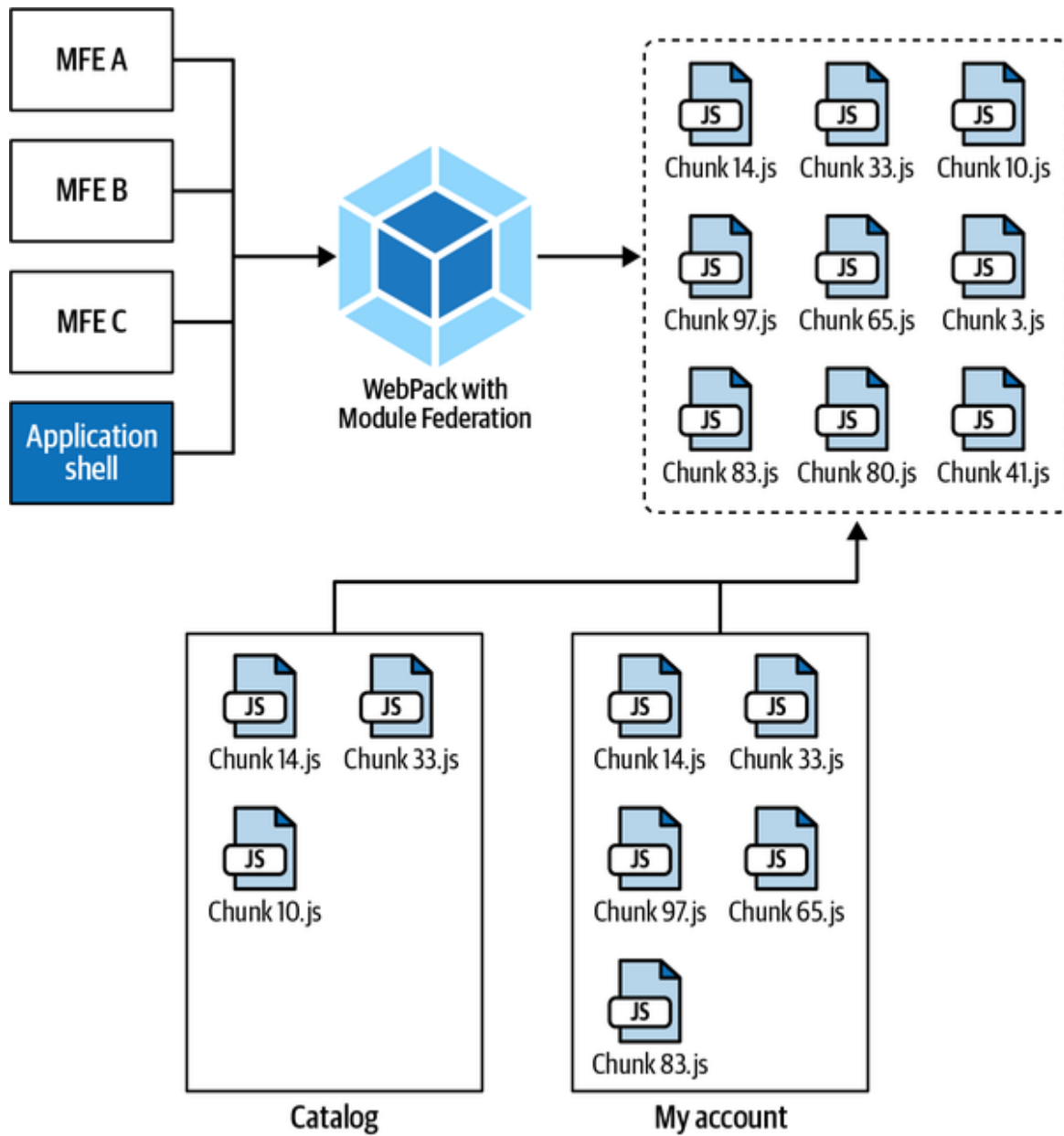
Figure 4-20. Module Federation allows multiple micro-frontends to be loaded asynchronously, providing the user with a seamless experience
