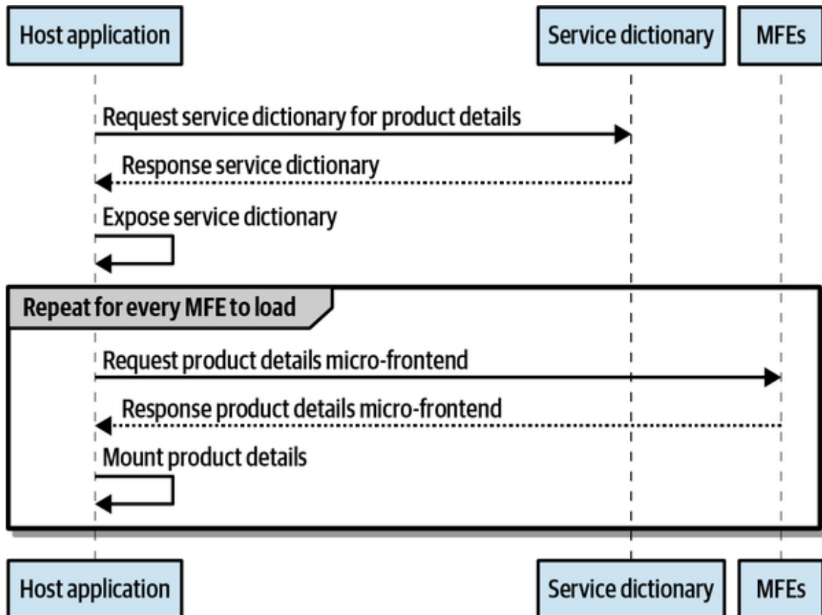
Figure 8-6. This sequence diagram shows how a horizontal-split architecture with client-side composition may consume the service dictionary API
