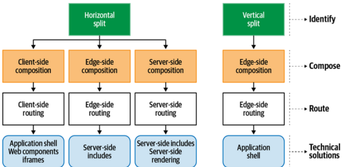
Figure 4-1. The micro-frontends decisions framework
