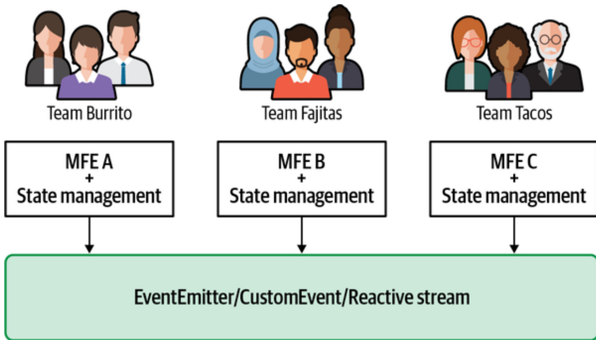
Figure 4-15. Every micro-frontend in the same view should own its own state and should communicate changes via asynchronous communication using an event emitter or CustomEvent or reactive streams
