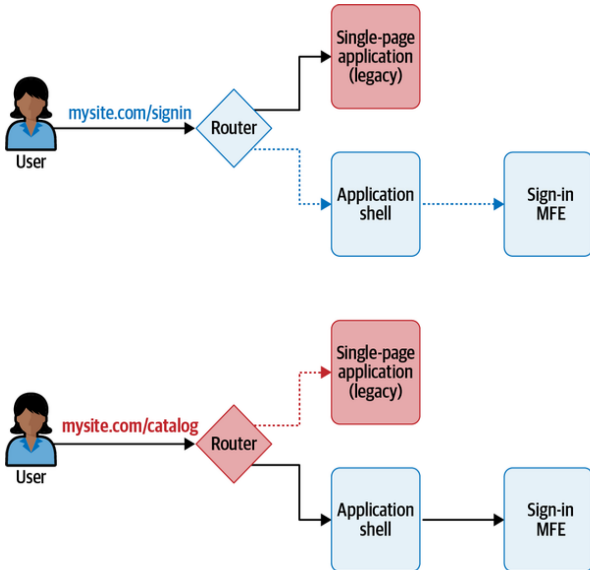
Figure 6-8. A strangler pattern where the micro-frontends live alongside the legacy application so that we can create immediate value for the users and the company instead of waiting for the entire application to be developed
