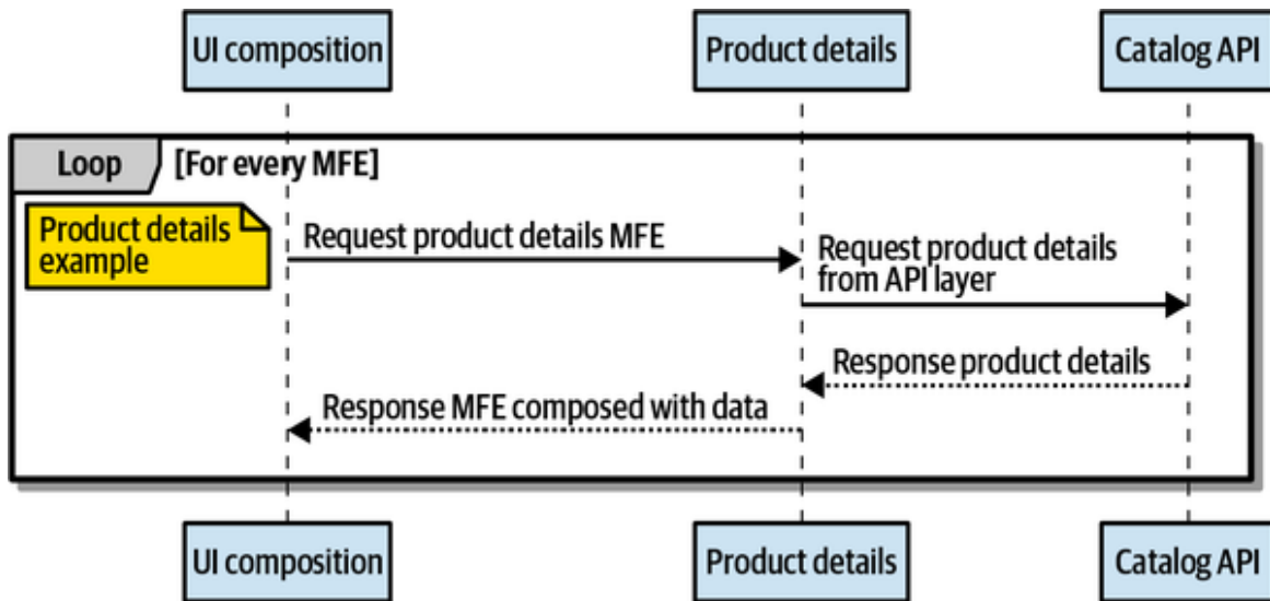
Figure 8-11. An example of server-side composition with API gateway
