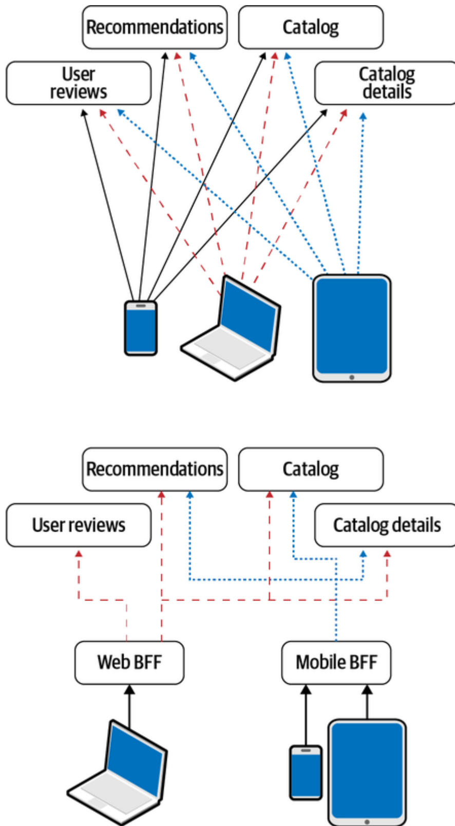
Figure 8-12. On the top, a microservices architecture consumed by different clients; on the bottom, a BFF layer exposing only the APIs needed for a given group of devices—in this case, mobile and web BFF
