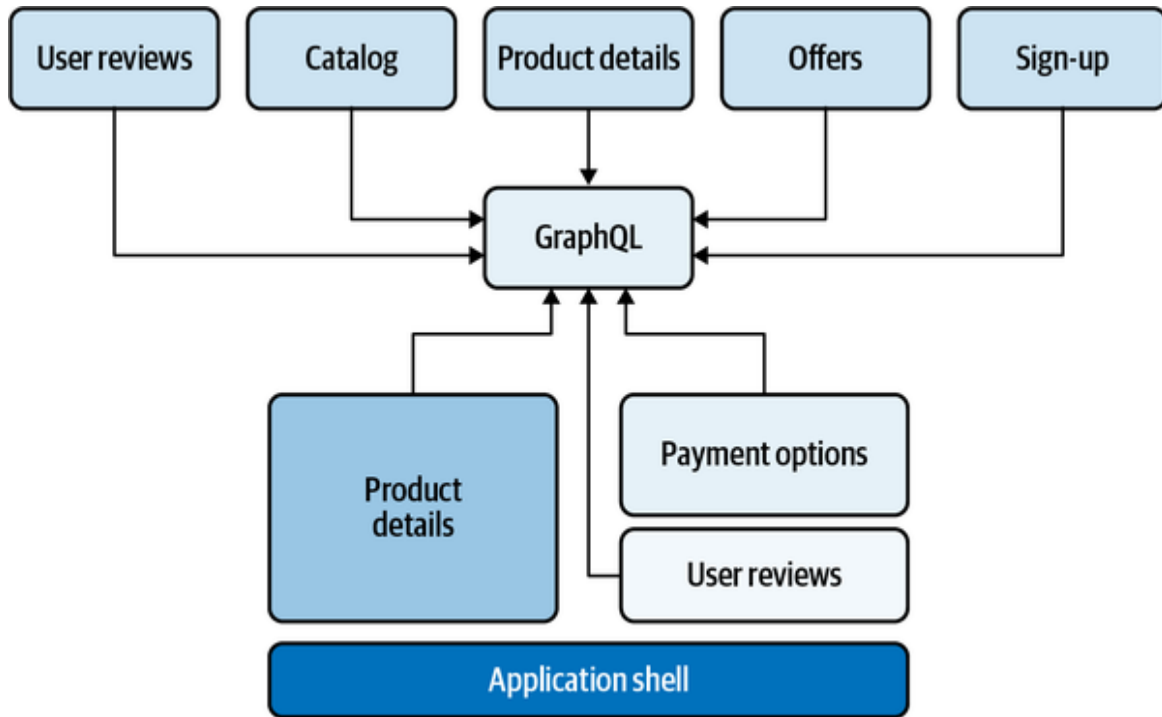
Figure 8-19. A high-level architecture of GraphQL with schema federation. When we implement it with a micro-frontend architecture with horizontal split and a client-side composition, all micro-frontends query the graph layer.
