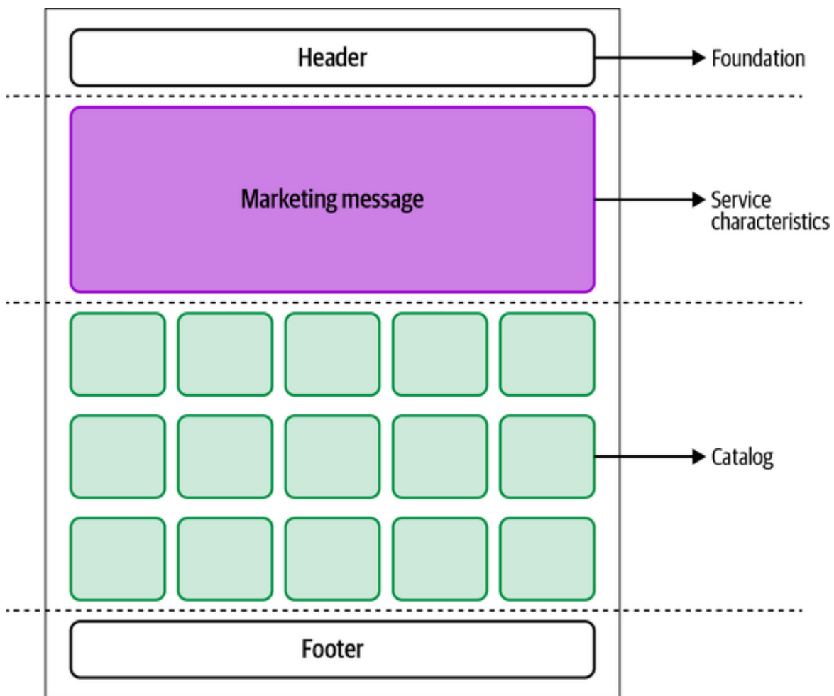
Figure 4-13. This new view is composed by the catalog (owned by the catalog team) and the marketing message (owned by the landing page team)
