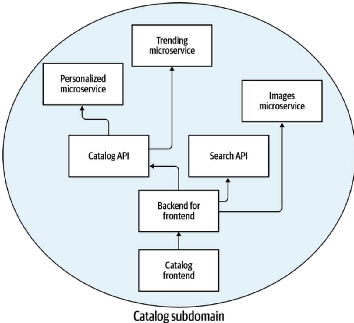
Figure 3-2. A representation of bounded context
