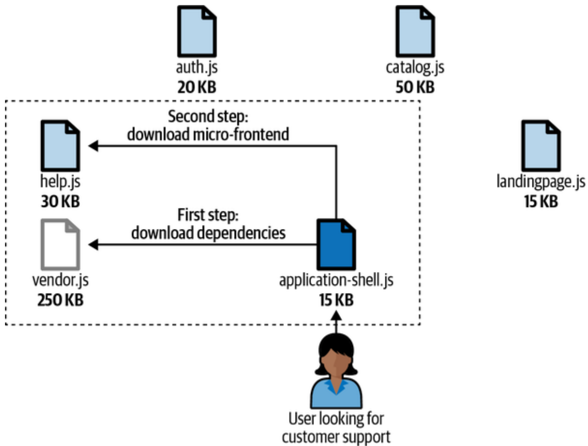
Figure 4-10. A vertical-split micro-frontend enables the user to download only the application code needed to accomplish the action the user is looking for
