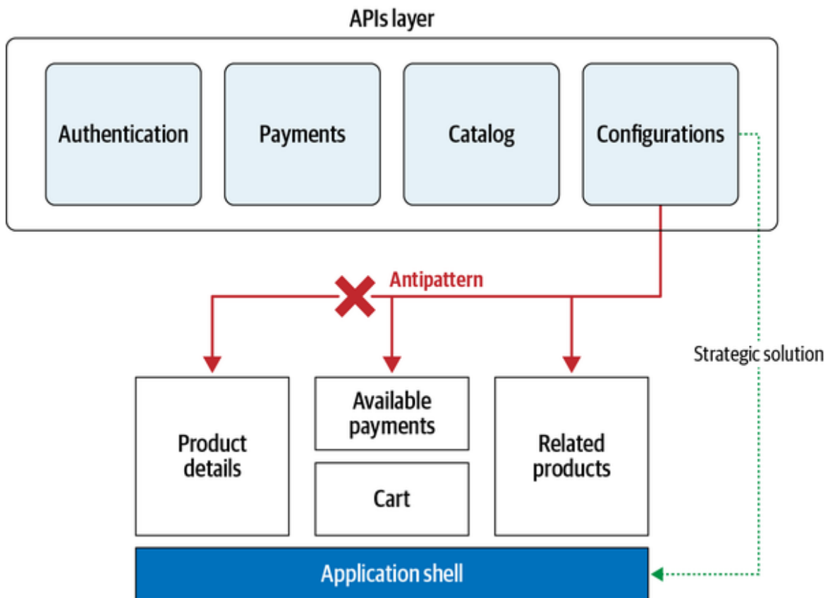
Figure 8-5. The service dictionary should always be loaded from the micro-frontend container in a horizontal-split architecture
