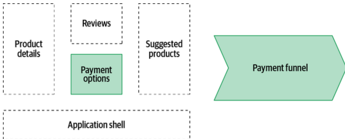
Figure 6-5. An end-to-end testing example with a horizontal-split architecture
