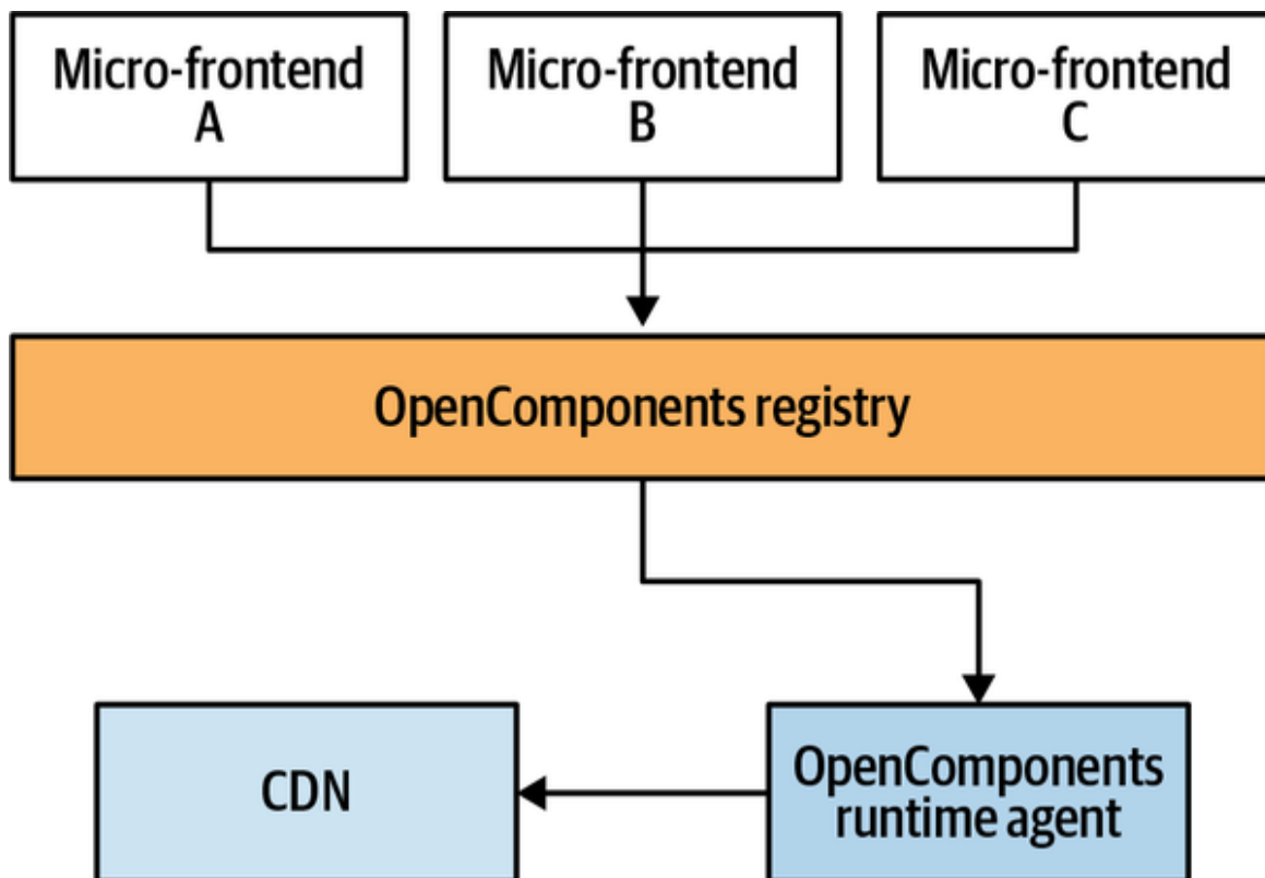
Figure 4-26. The OpenComponents architecture shows how a server-side rendered micro-frontend is flowing from development to an environment
