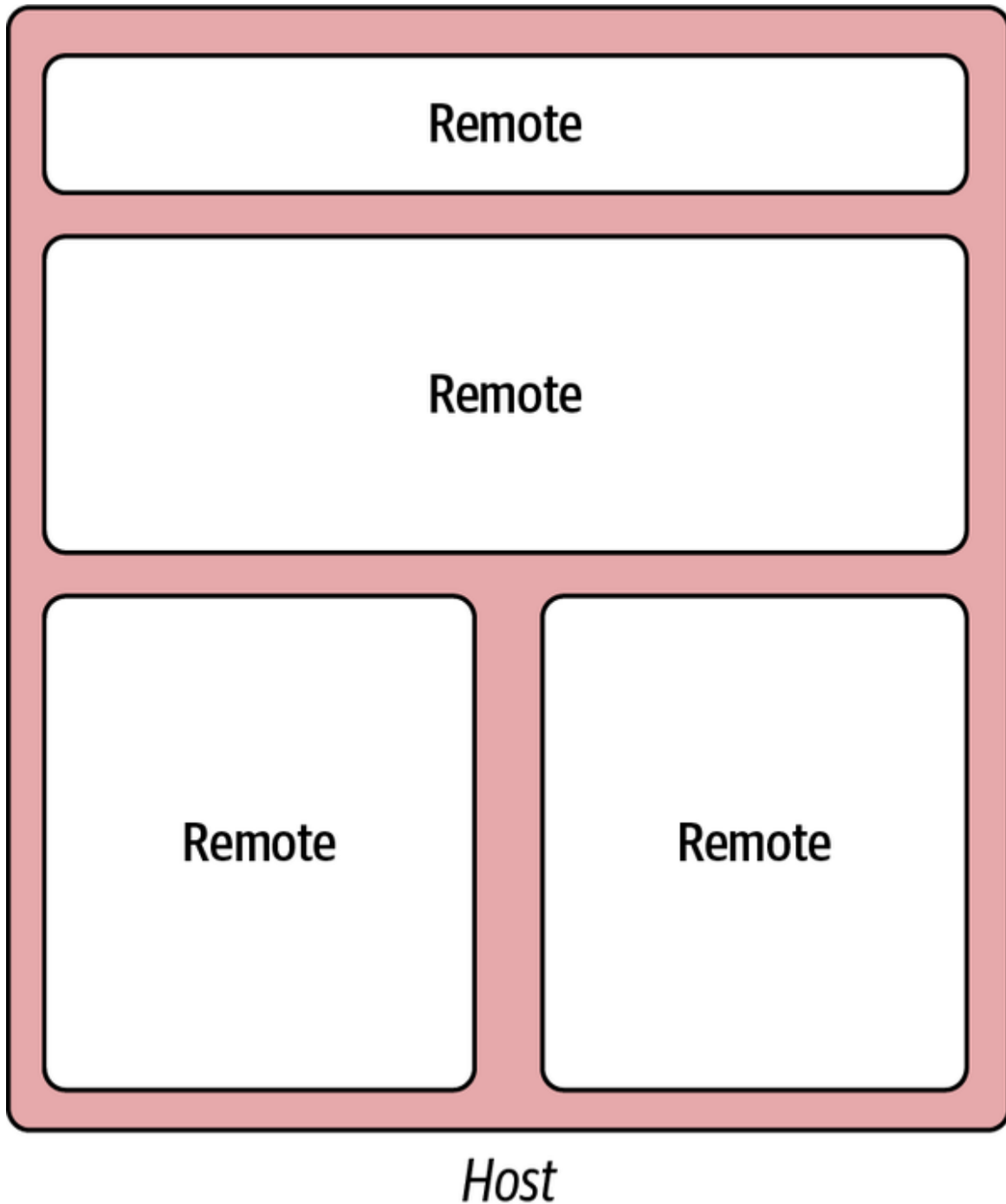
Figure 5-2. Module Federation is composed of two key elements: the host, which is responsible for loading some JavaScript bundles at runtime, and the remote, which is responsible for any type of JavaScript bundles, such as shared libraries, micro-frontends, or even components
