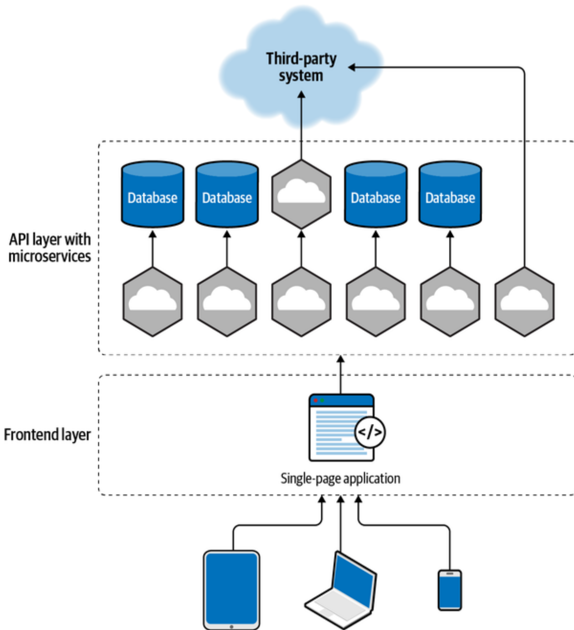
Figure 2-2. Microservices with single-page application
