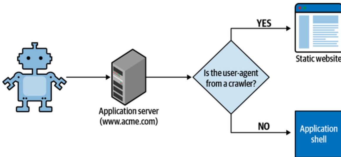
Figure 4-8. When a crawler requests a specific page, the application server should retrieve the user-agent and serve the crawler's requests to a prerendered version of the website, otherwise serving the micro-frontend implementation
