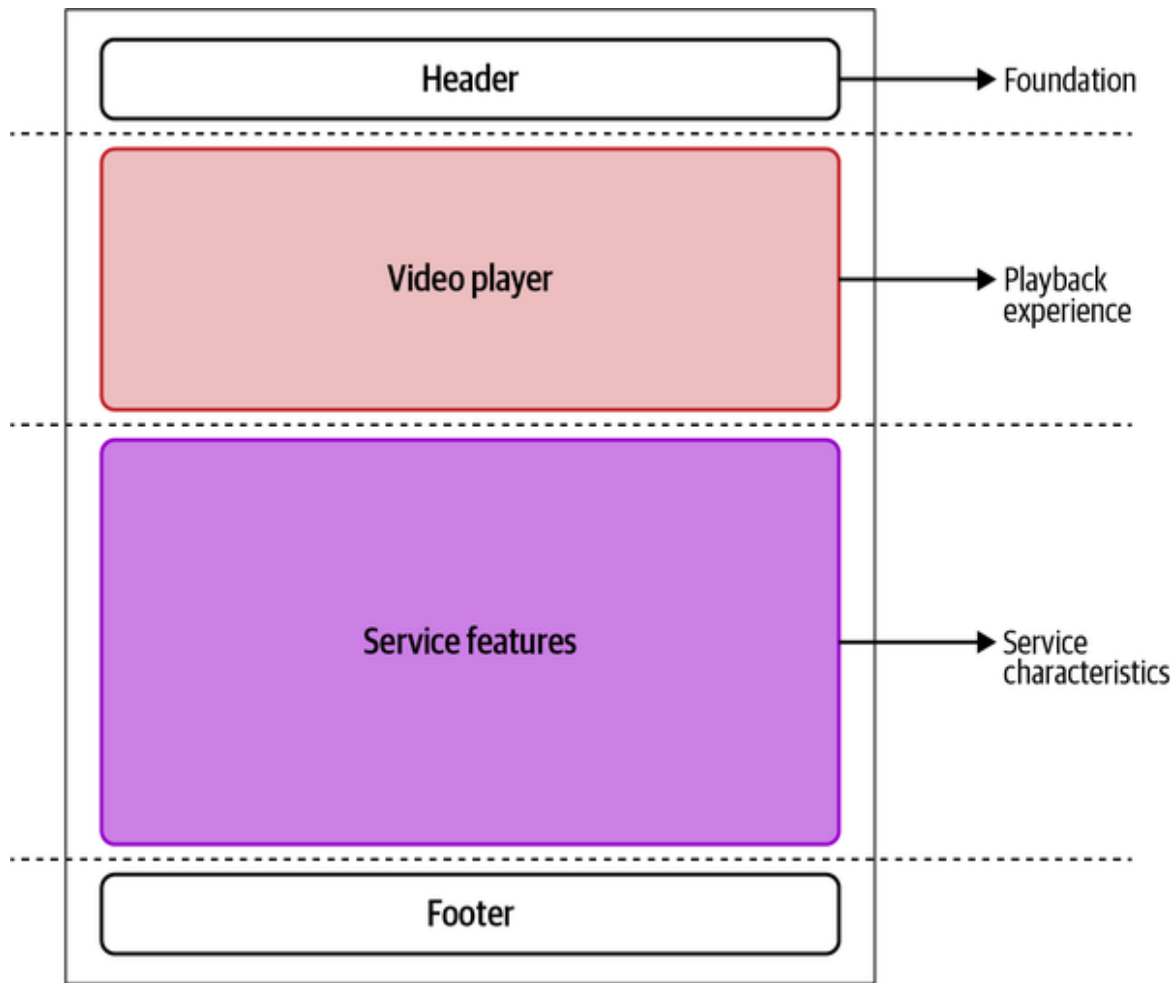
Figure 4-11. The landing page view is composed by the application shell, which loads two micro-frontends: the service characteristics and the playback experience
