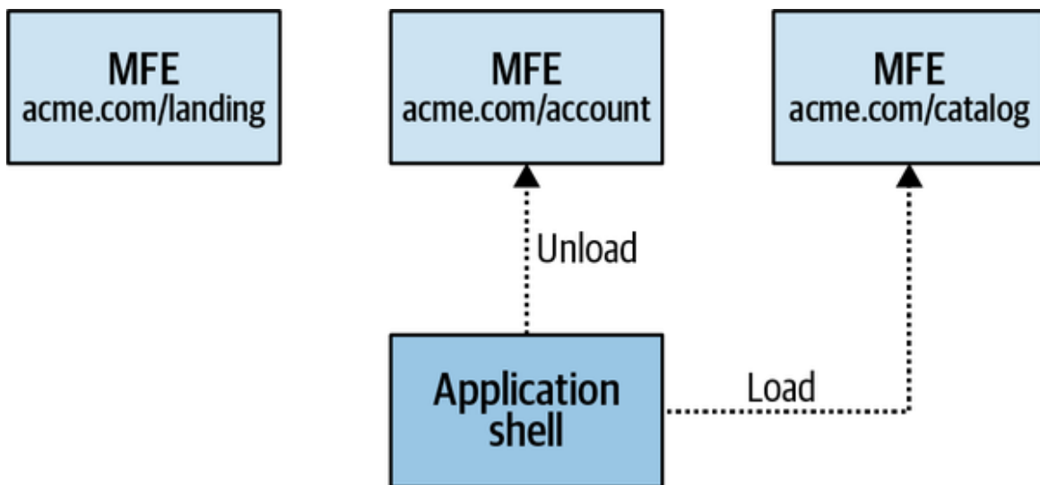
Figure 9-7. When the user signs in from the /account path, they are redirected to the authenticated area (/catalog). The application shell owns the logic for unloading the current micro-frontend and loading the next one based on the URL.
