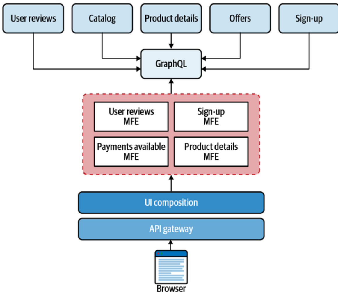
Figure 8-20. A high-level architecture for a micro-frontend architecture with a server-side composition where every micro-frontend consumes the graph exposed by the GraphQL server
