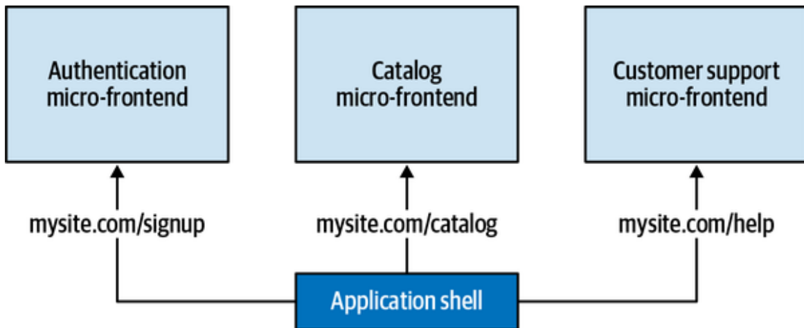
Figure 4-2. The application shell is responsible for global routing between micro-frontends
