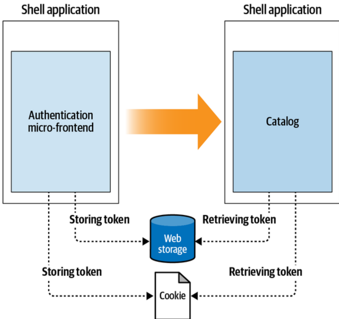
Figure 3-6. Sharing data between micro-frontends in different views
