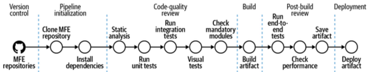
Figure 7-6. The end-to-end automation strategy diagram
