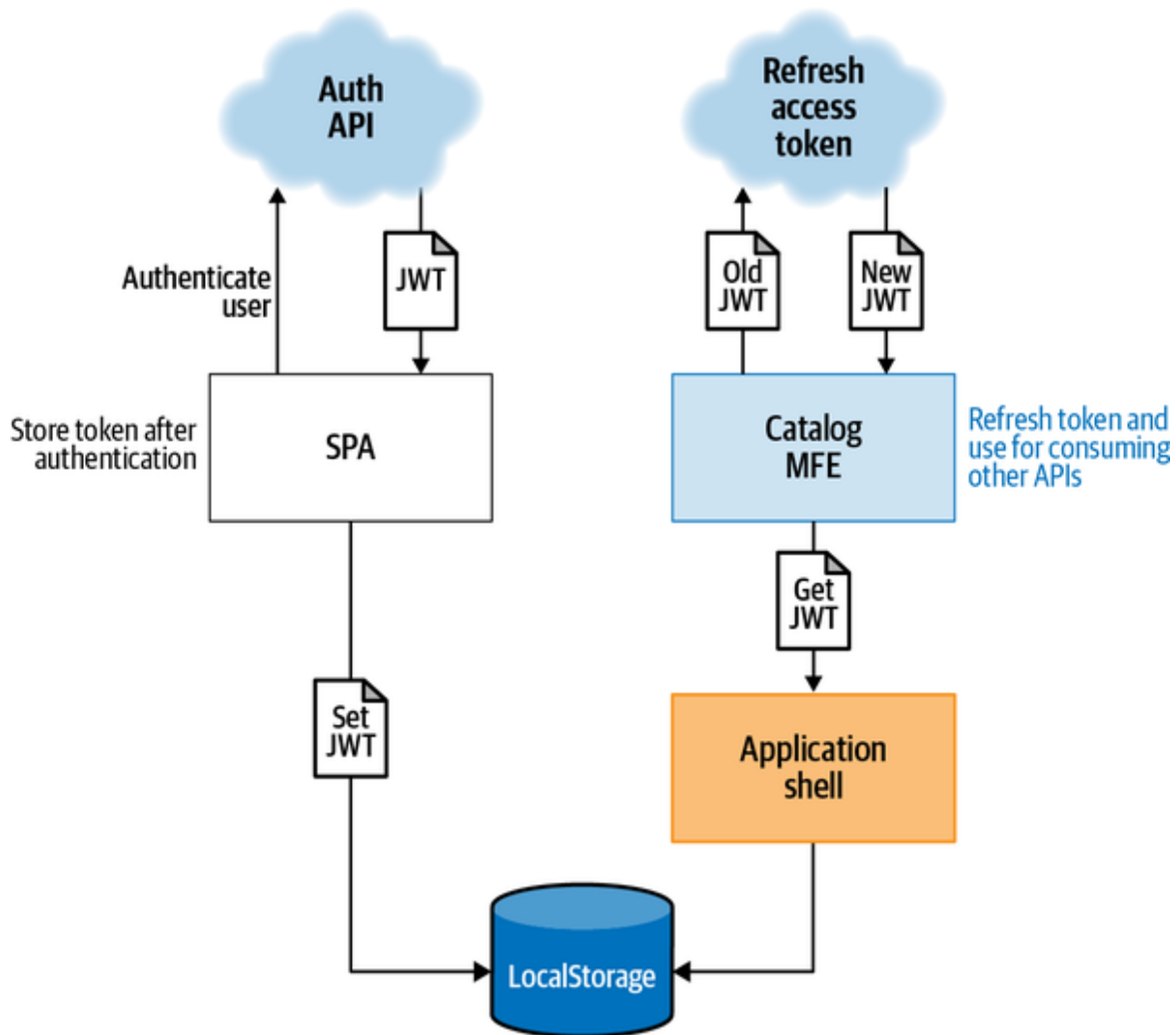
Figure 9-12. During the migration, the SPA authenticates a user and stores the token in the local storage, which the authenticated micro-frontend retrieves once loaded
