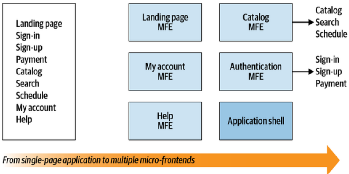
Figure 9-9. Migration path: from SPA to micro-frontends
