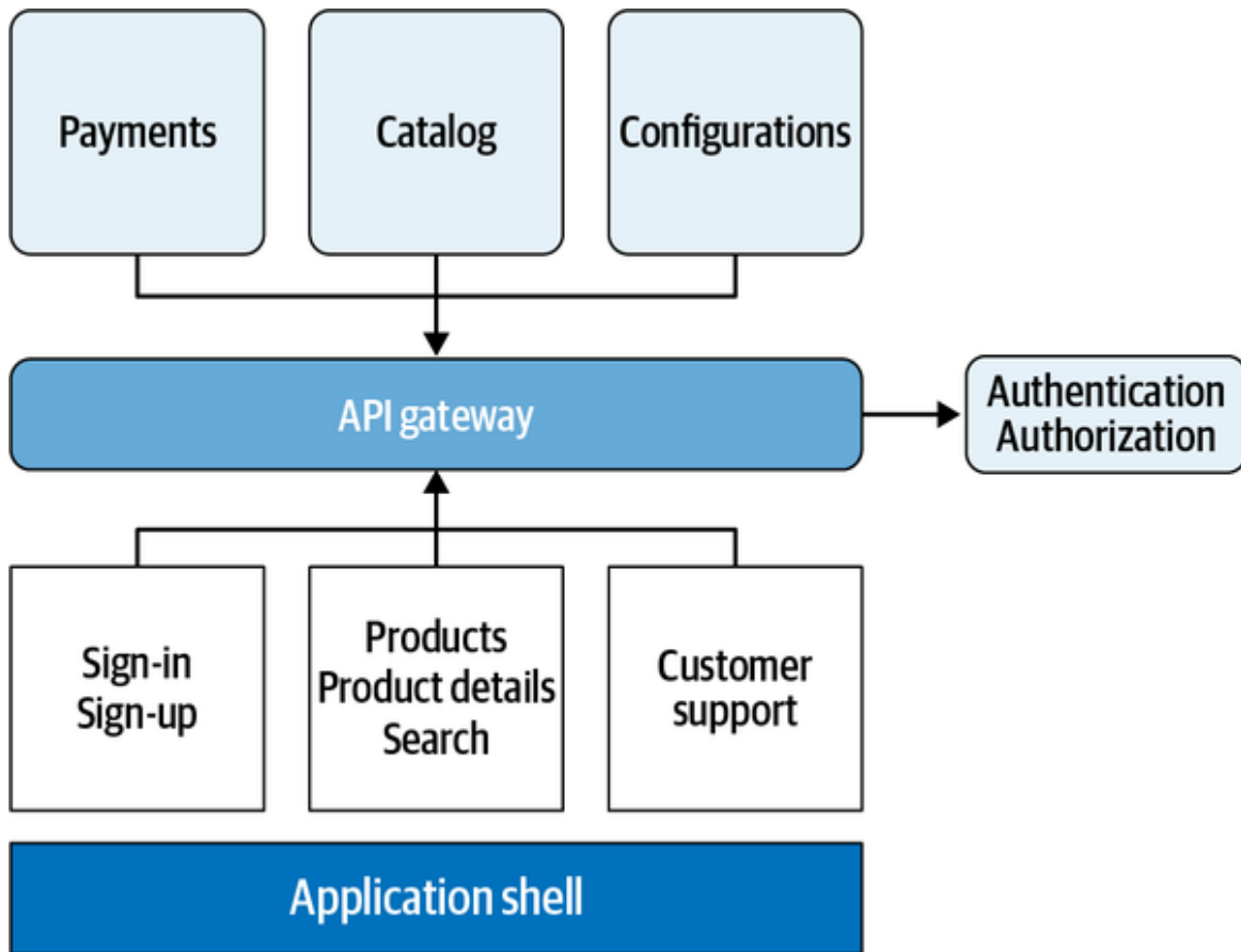
Figure 8-9. A vertical-split architecture with a client-side composition requesting data to a microservice architecture with an API gateway as entry point
