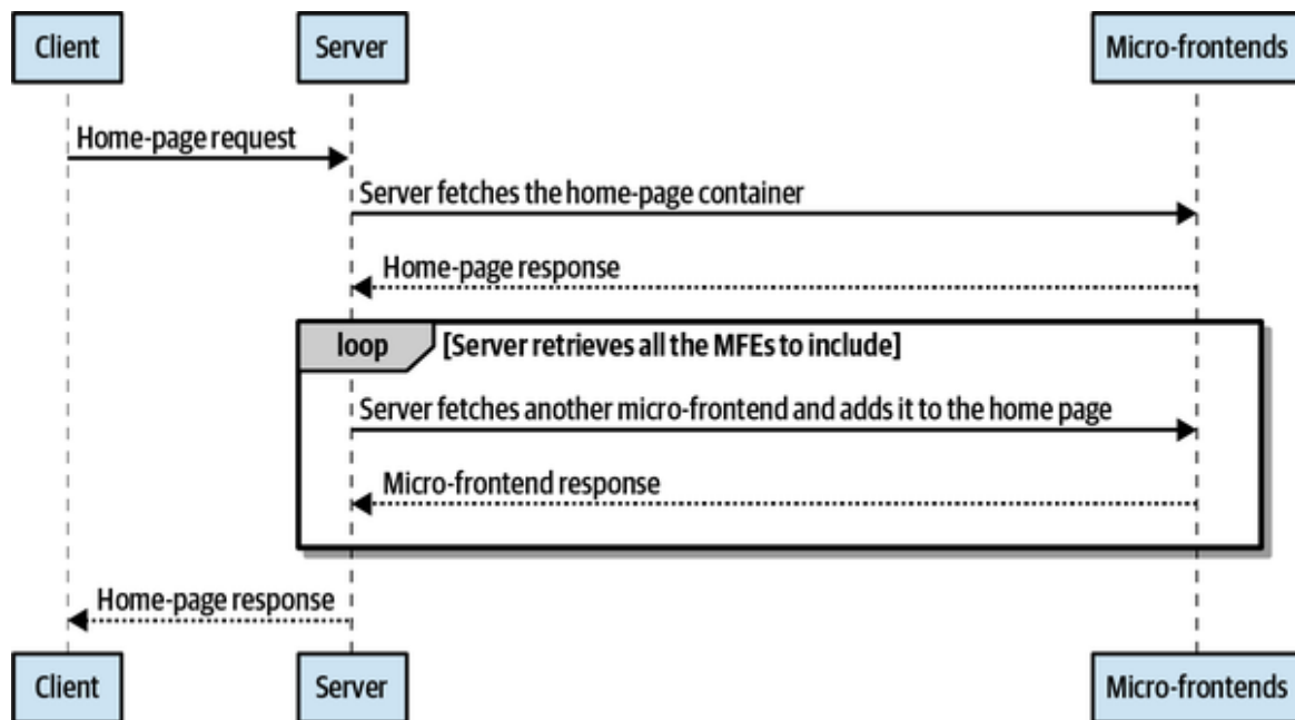
Figure 4-27. The sequence diagram shows how a client request is handled by a server when SSI are used
