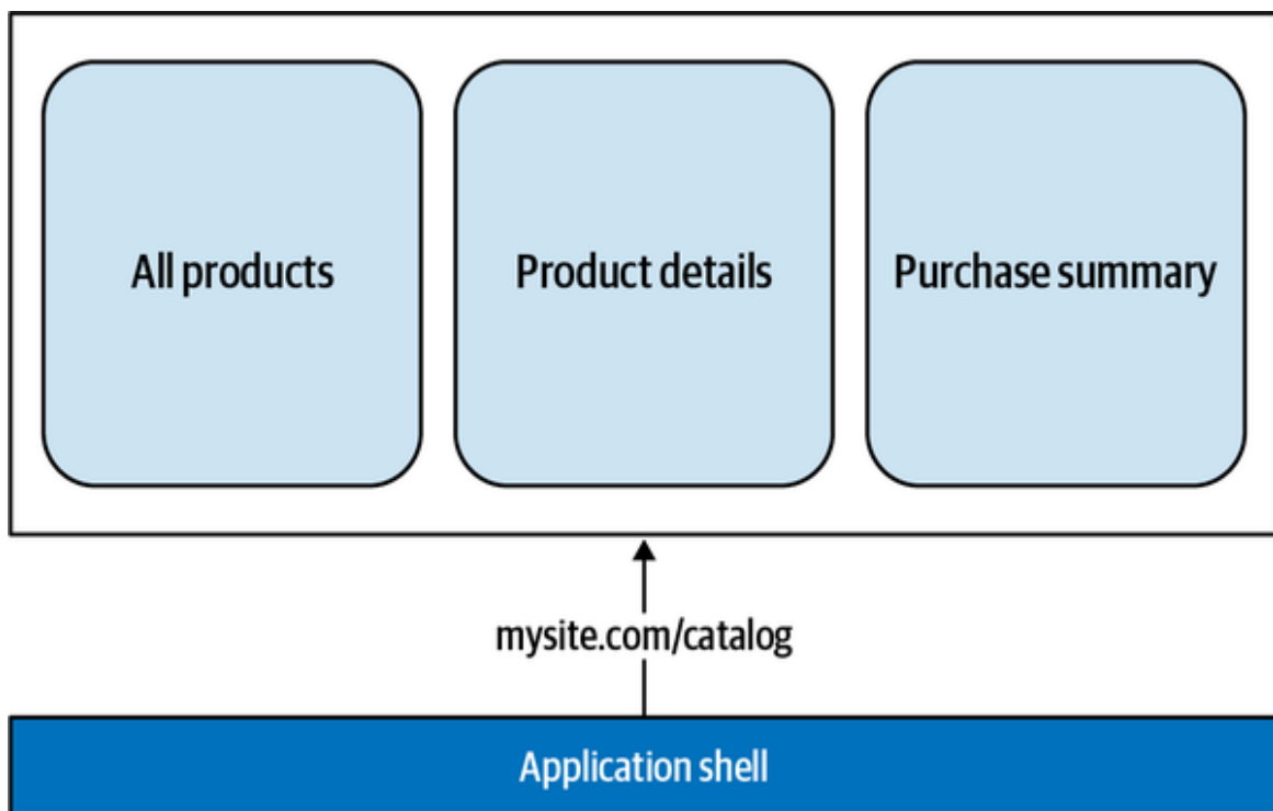
Figure 4-3. A micro-frontend is responsible for routing between views available inside the micro-frontend itself
