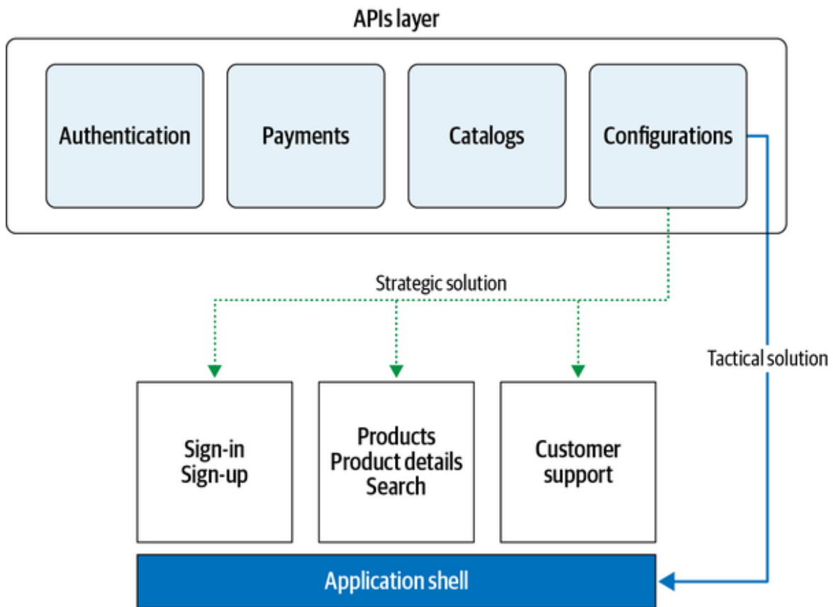
Figure 8-3. With vertical-split architecture, we can retrieve the service dictionary directly inside a micro-frontend from an endpoint—in this case, Configurations . Dividing the endpoints list by business domain allows us to structure our teams accordingly.
