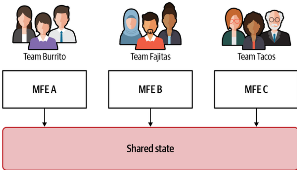
Figure 4-14. Shared state between multiple micro-frontends represents an antipattern
