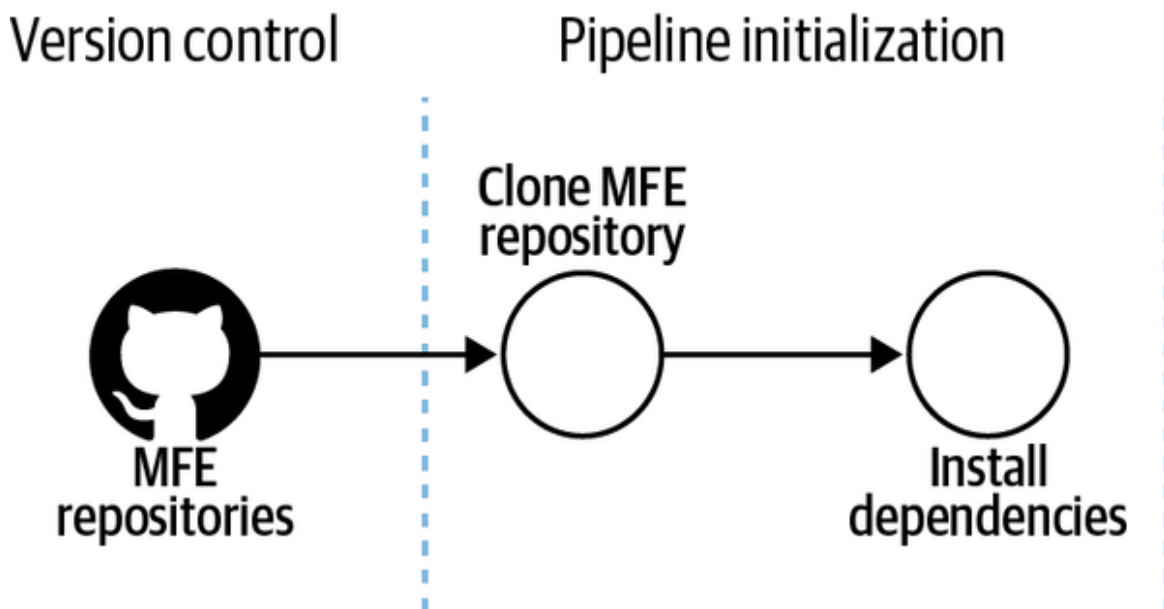
Figure 7-3. Pipeline initialization stage, showing two actions: cloning the repository and installing the dependencies
