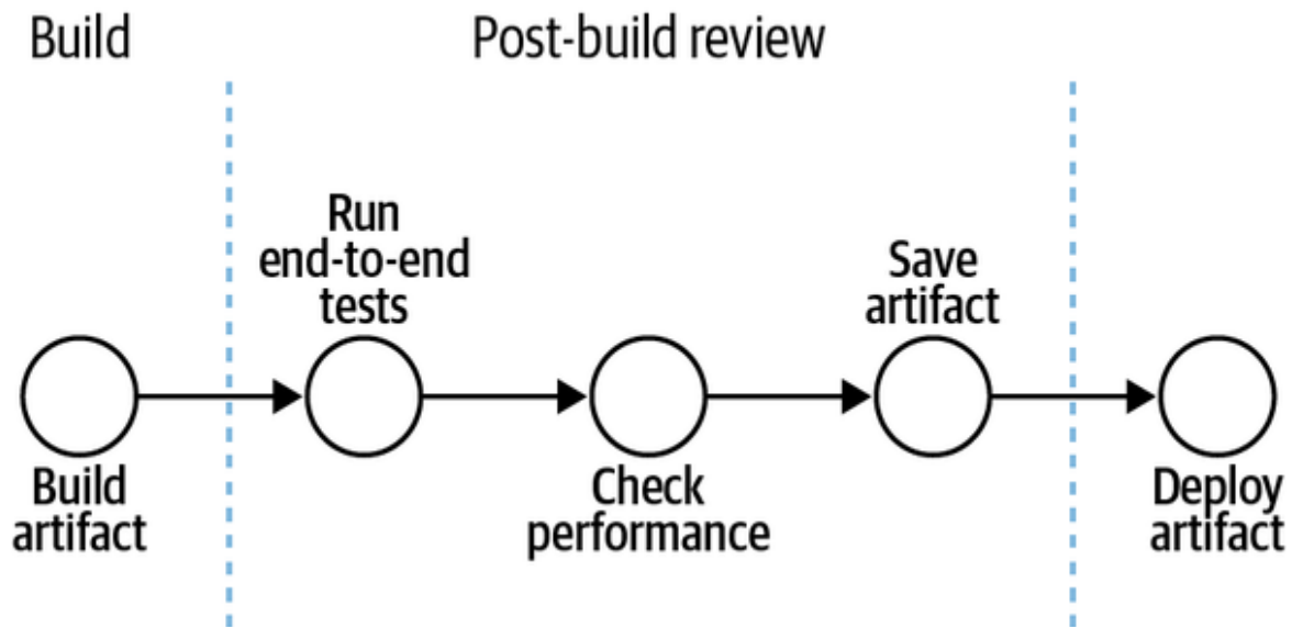
Figure 7-5. In the post-build review, we perform additional checks before deploying an artifact to an environment
