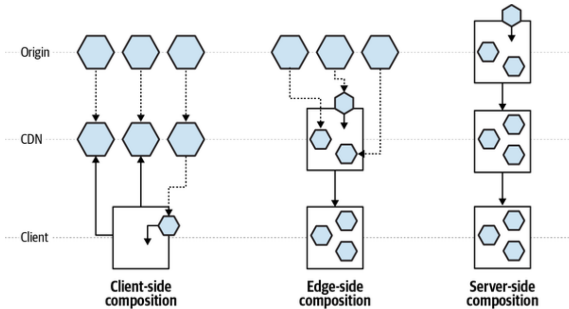
Figure 3-3. Micro-frontends composition diagram
