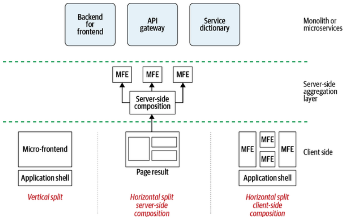
Figure 8-1. Micro-frontends and API layers
