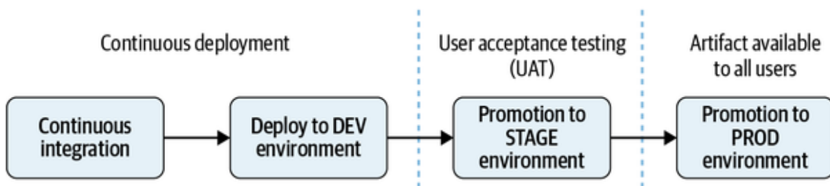
Figure 7-1. An example of an environments strategy
