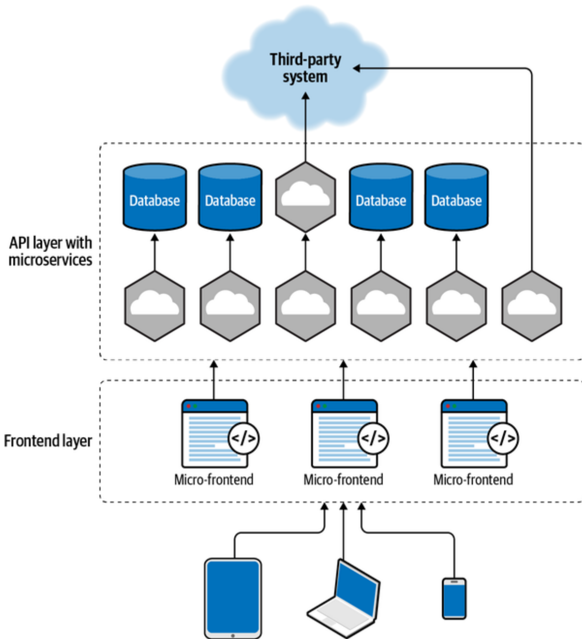
Figure 2-3. Microarchitectures combined. This is a high-level diagram showing how microservices and micro-frontends can live together.
