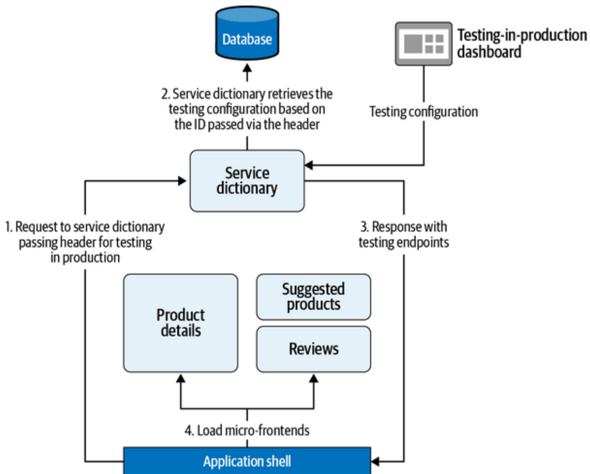
Figure 8-2. A high-level architecture on how to use a service dictionary for testing in production
