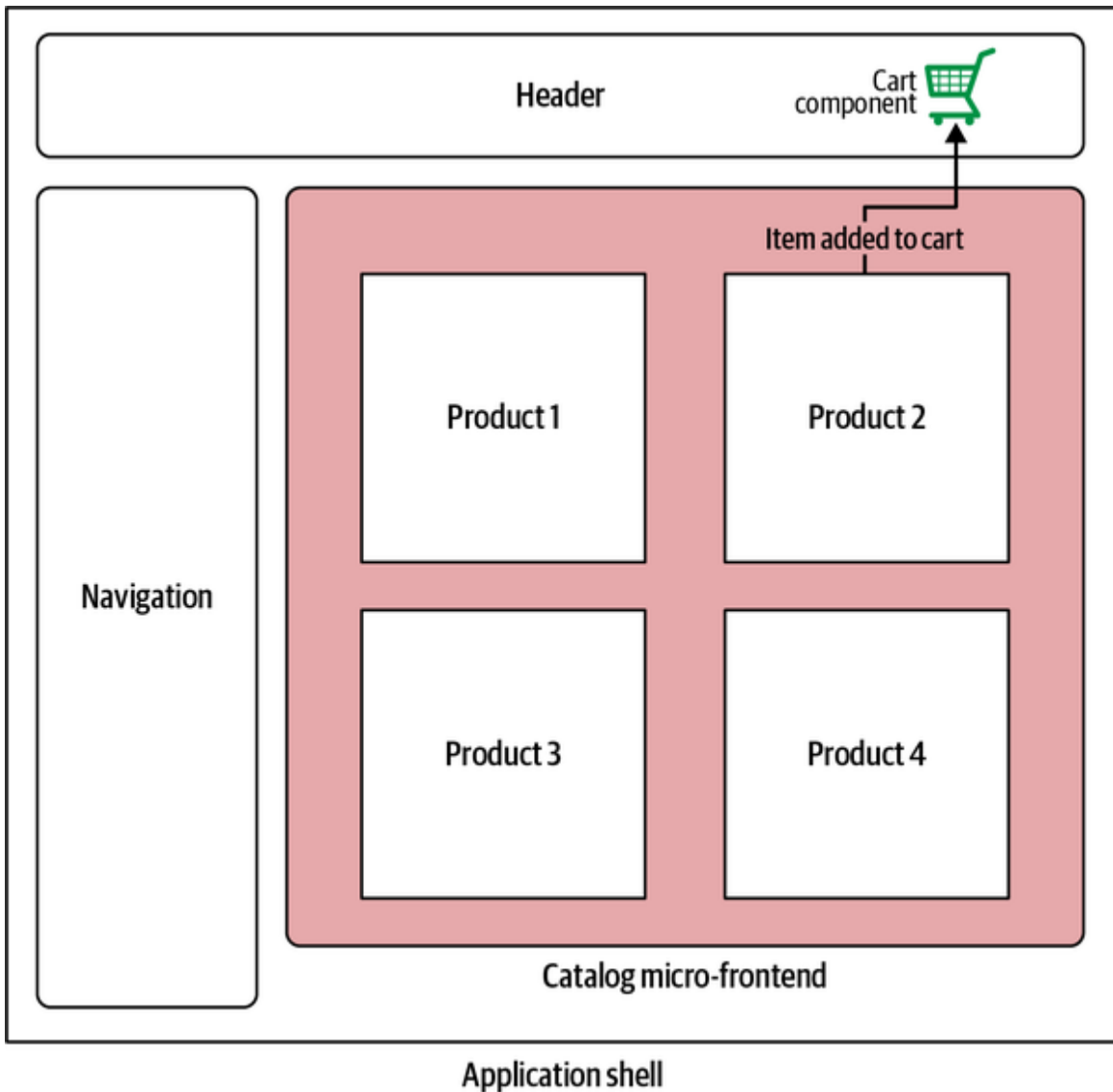
Figure 5-7. The cart component is created and maintained by Team Nigiri. The component is loaded inside the application shell and uses an event emitter for listening for when an object should be added to the cart and showing the total number of elements the user has selected.
