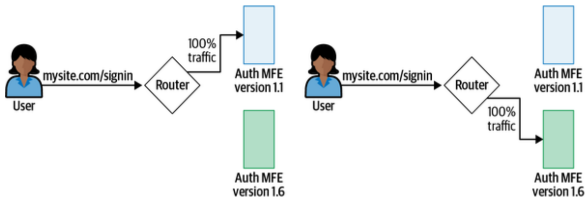
Figure 6-6. Blue-green deployment
