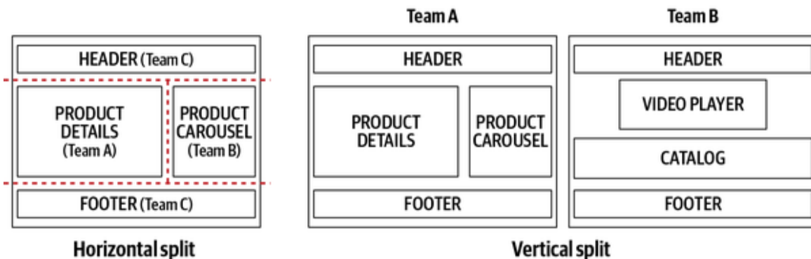
Figure 3-1. Horizontal versus vertical split
