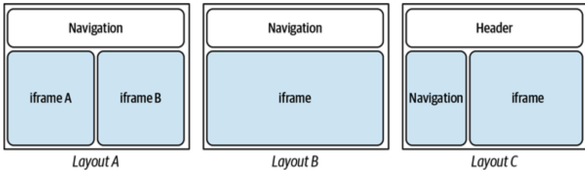
Figure 4-21. Different layouts for composing micro-frontends with iframes. Minimizing the number of iframes in a page would result in better performance despite there being an intrinsic performance overhead when we integrate one or more iframes into a view.
