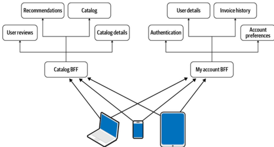
Figure 8-14. This diagram shows how to separate different domain-driven design subdomains
