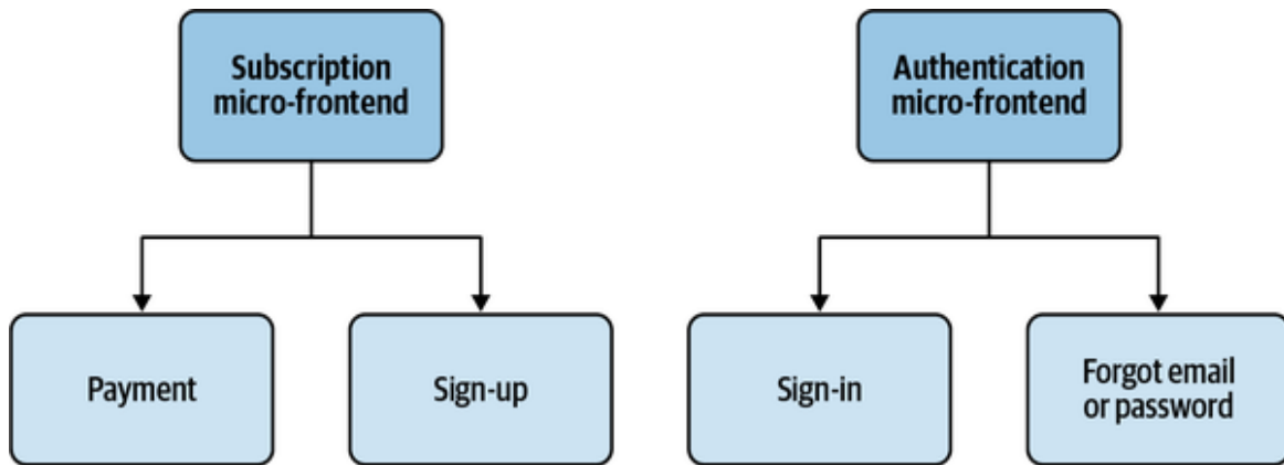
Figure 4-6. Splitting the authentication micro-frontend to reduce the cognitive load, following customer experience more than technical constraints
