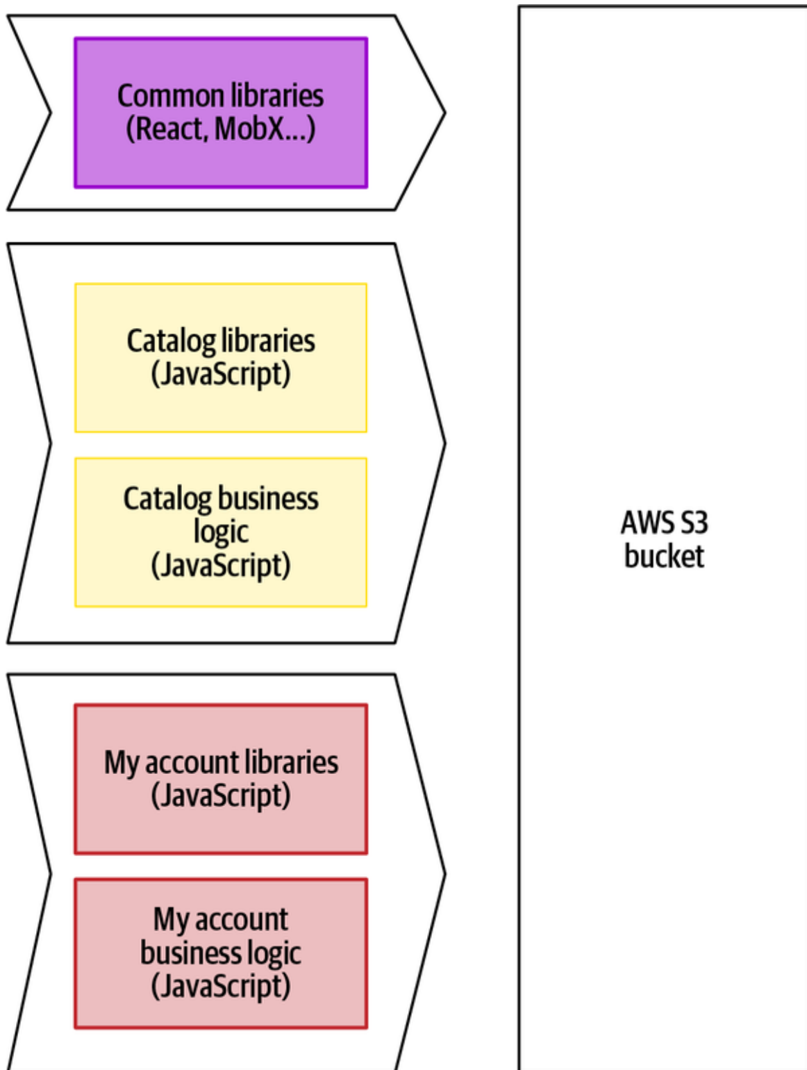
Figure 9-14. Every micro-frontend builds and deploys its own JavaScript dependencies, apart from the common libraries, which have a separate automation strategy
