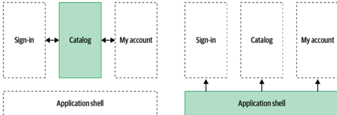
Figure 6-4. An end-to-end testing example with a vertical split architecture
