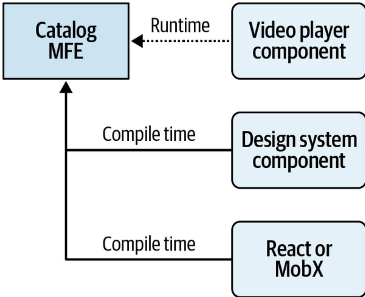
Figure 9-15. In a micro-frontend, complex components owned by a single team are loaded at runtime, while all the others are embedded at compile time. The only exception is the design system due to its modular nature.
