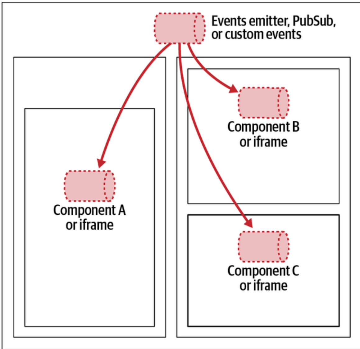
Figure 3-5. Event emitter and custom events diagram
