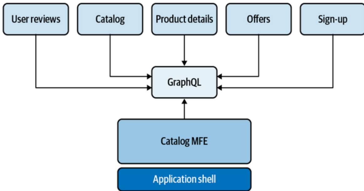
Figure 8-18. A high-level architecture for composing a microservice backend with schema federation. The catalog micro-frontend consumes the graph composed by all the schemas inside the GraphQL server.
