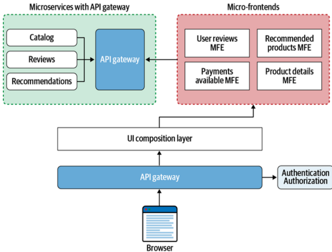
Figure 8-10. An example of a server-side composition with a microservices architecture
