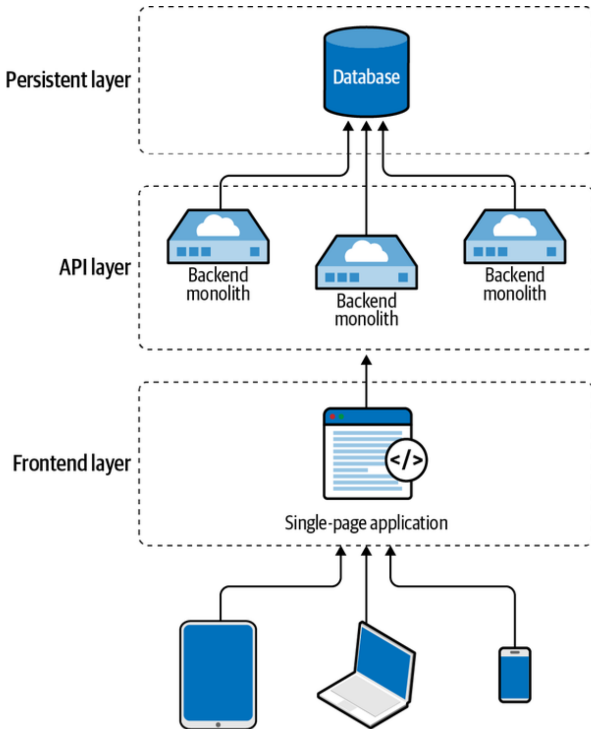
Figure 2-1. Monolith application with single-page application
