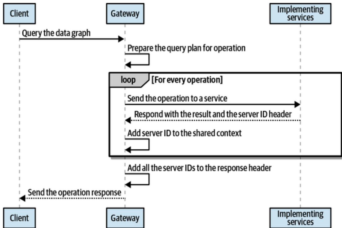
Figure 8-17. A sequence diagram showing how schema federation exposes all the schemas from multiple services
