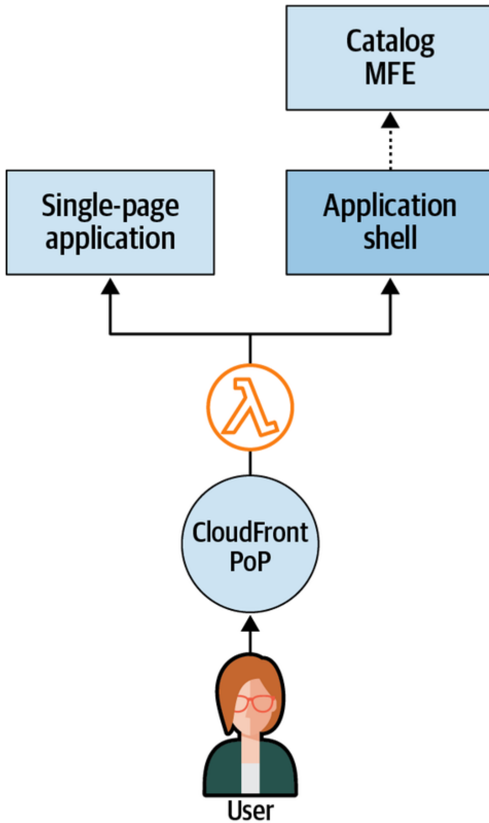
Figure 9-11. Strangler pattern applied at the infrastructure level using Lambda@Edge for funneling the traffic toward either the legacy or micro-frontend application
