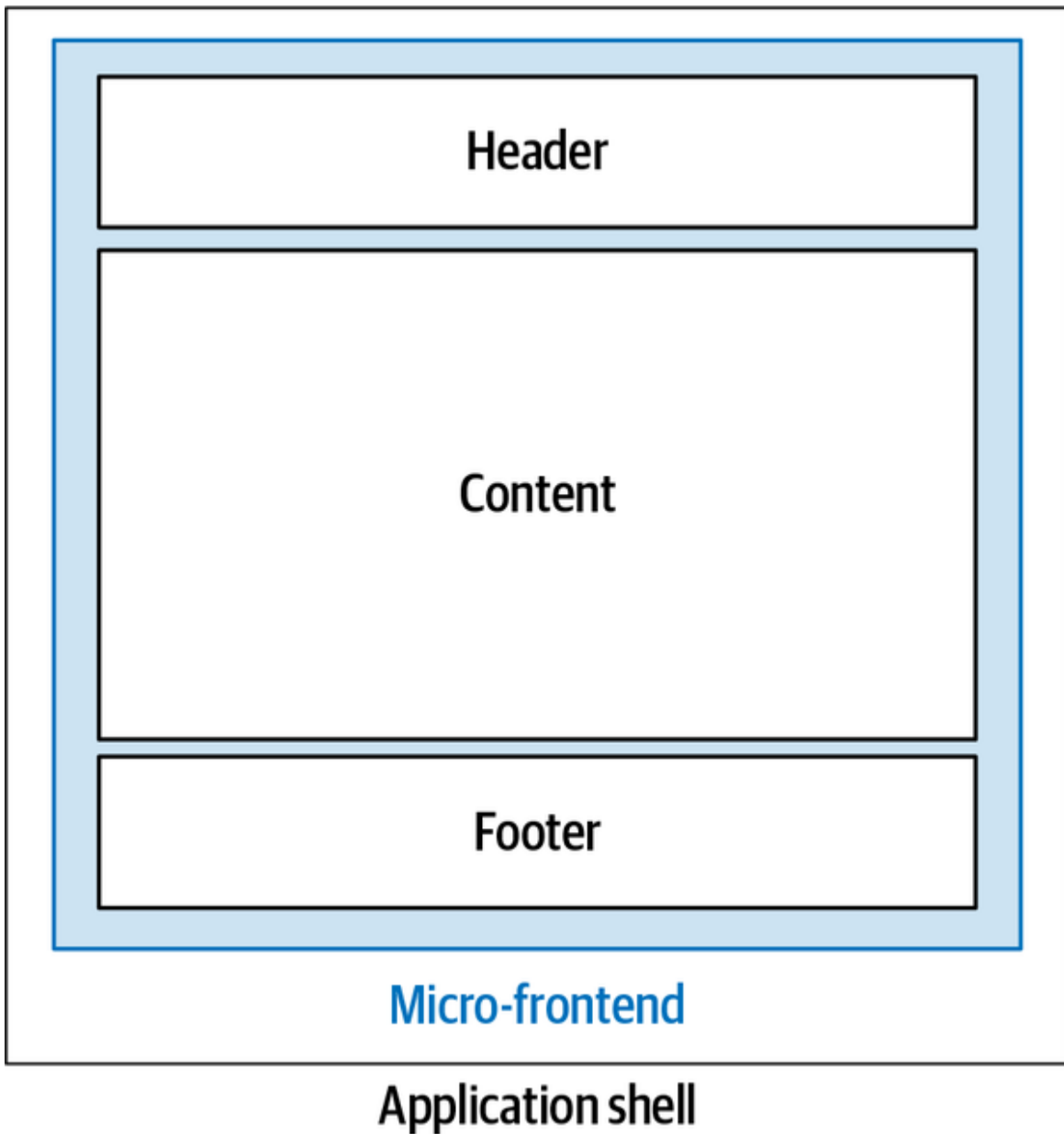
Figure 9-5. A vertical-split micro-frontend, where the application shell loads only one micro-frontend at a time
