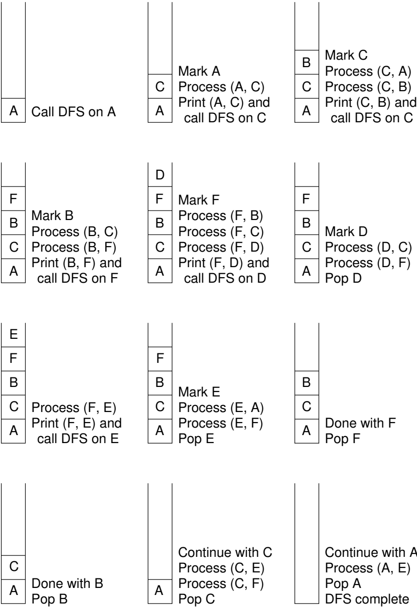
Figure 11.9 A detailed illustration of the DFS process for the graph of Figure 11.8(a) starting at Vertex A. The steps leading to each change in the recursion stack are described.
