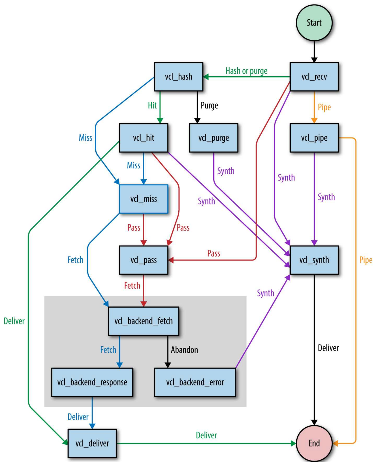
Figure 4-1. The simplified flow of execution in Varnish
