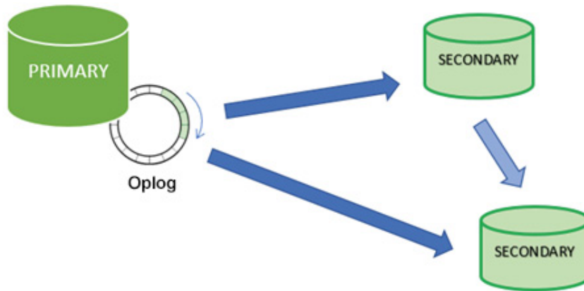
Figure 10.3: MongoDB replication
