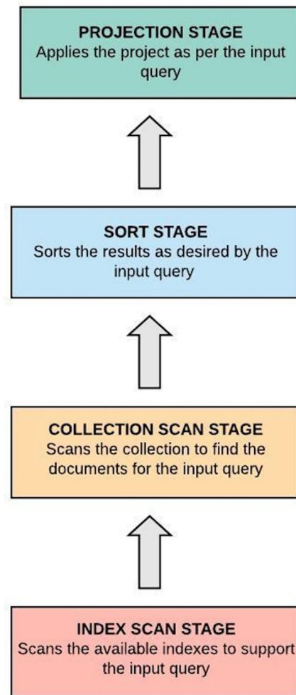
Figure 9.1: Query execution stages
