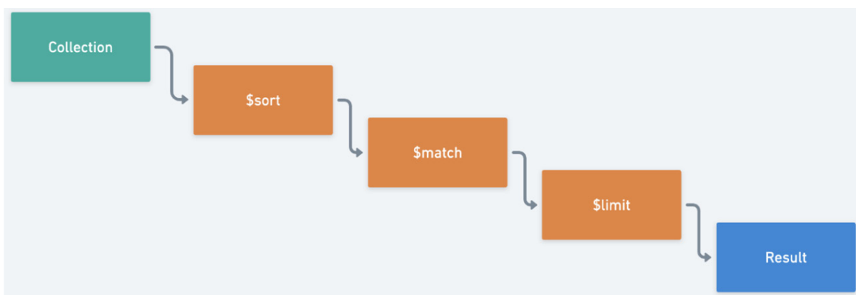
Figure 7.2: Aggregation pipeline
