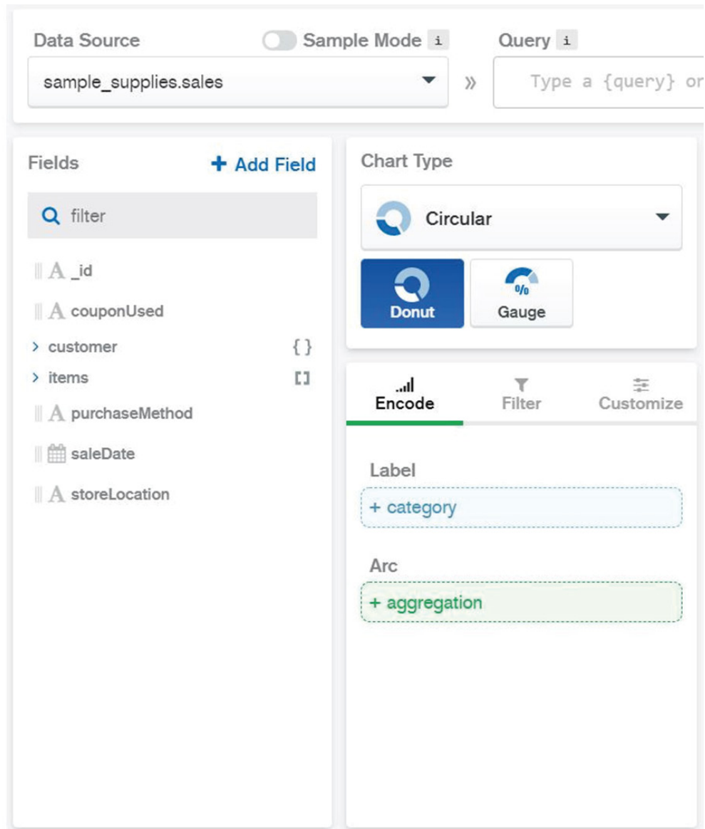
Figure 12.55: Selecting the Circular chart type and the Donut chart sub-type
