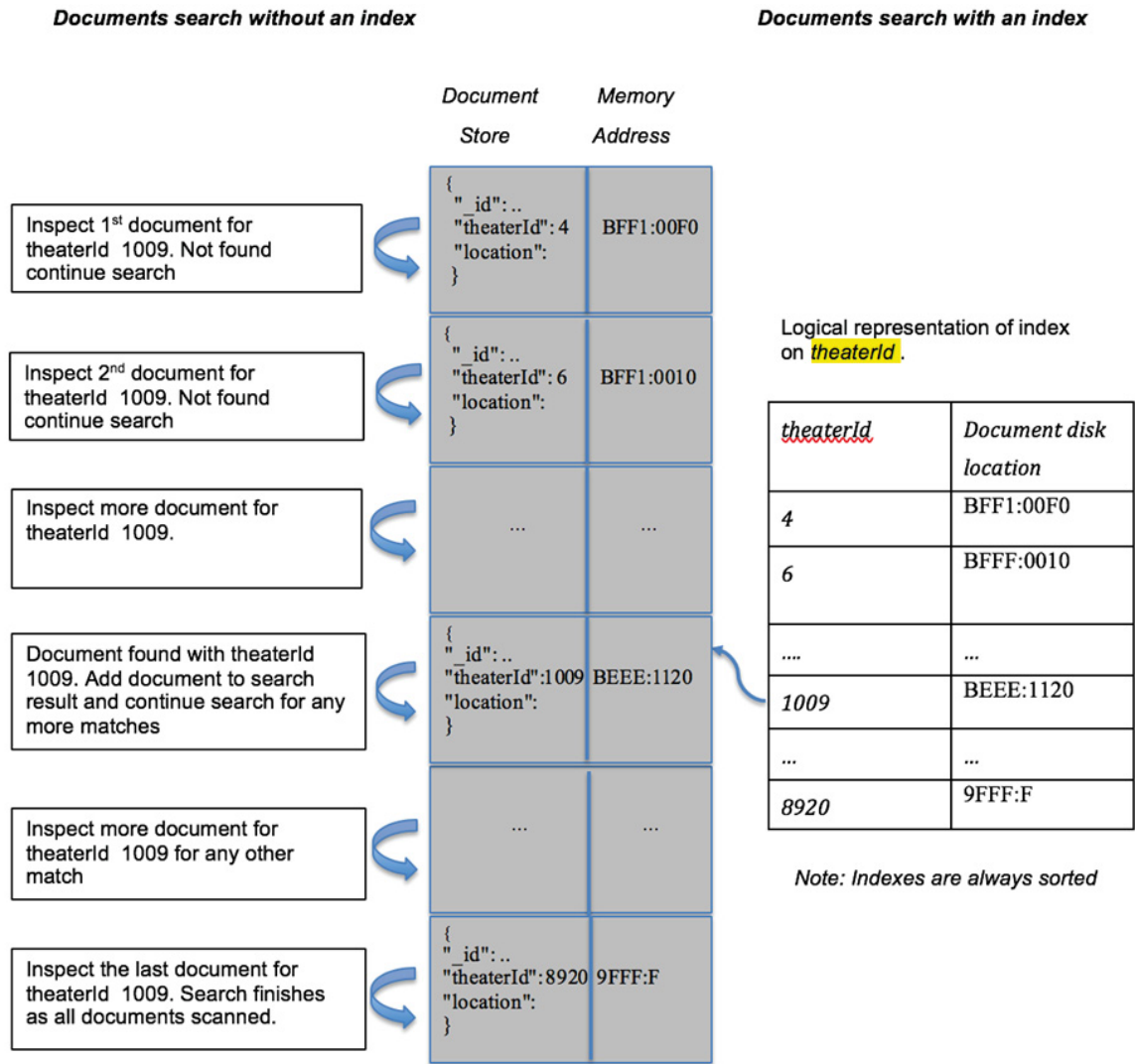
Figure 9.2: Data search with and without an index
