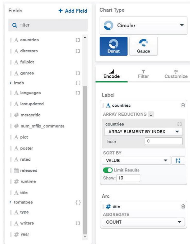
Figure 12.26: Setting the value of Limit Results to 10
