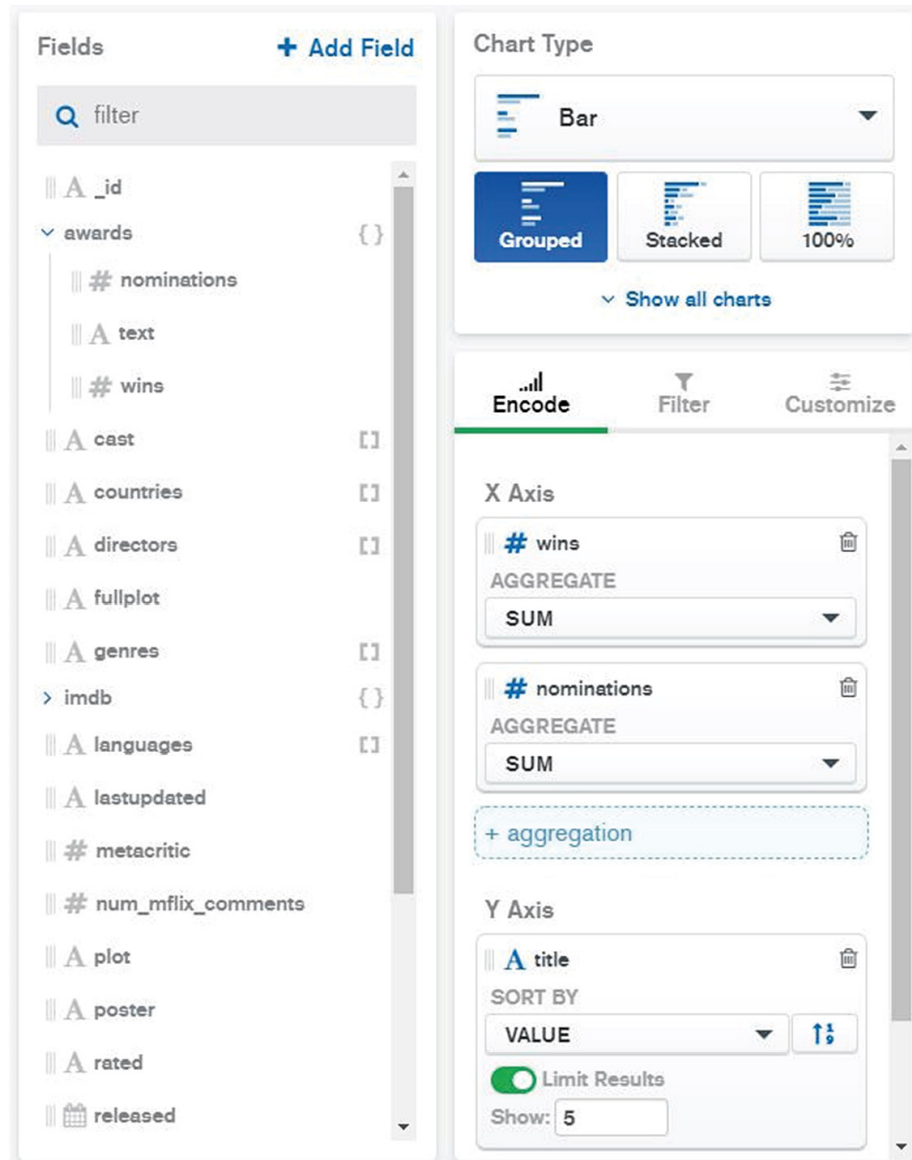
Figure 12.21: Dragging the nominations field to X Axis
