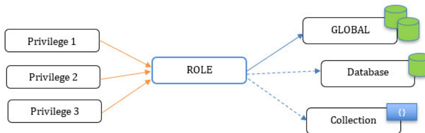
Figure 3.22: Pictorial representation of database privileges
