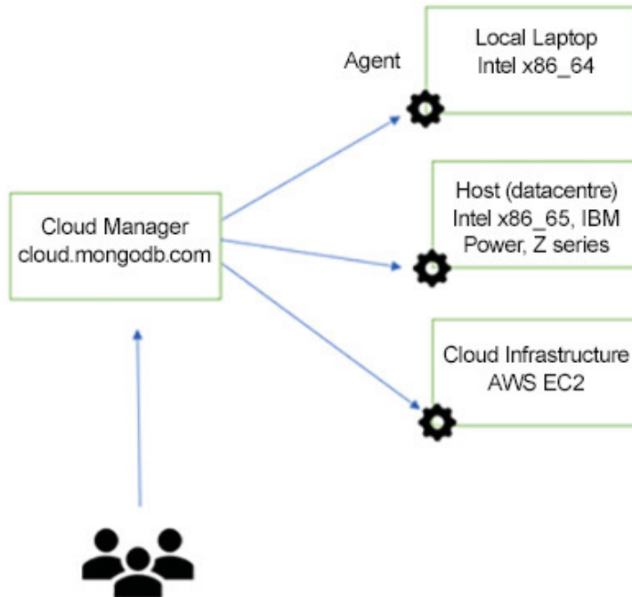
Figure 10.24: Cloud Manager architecture
