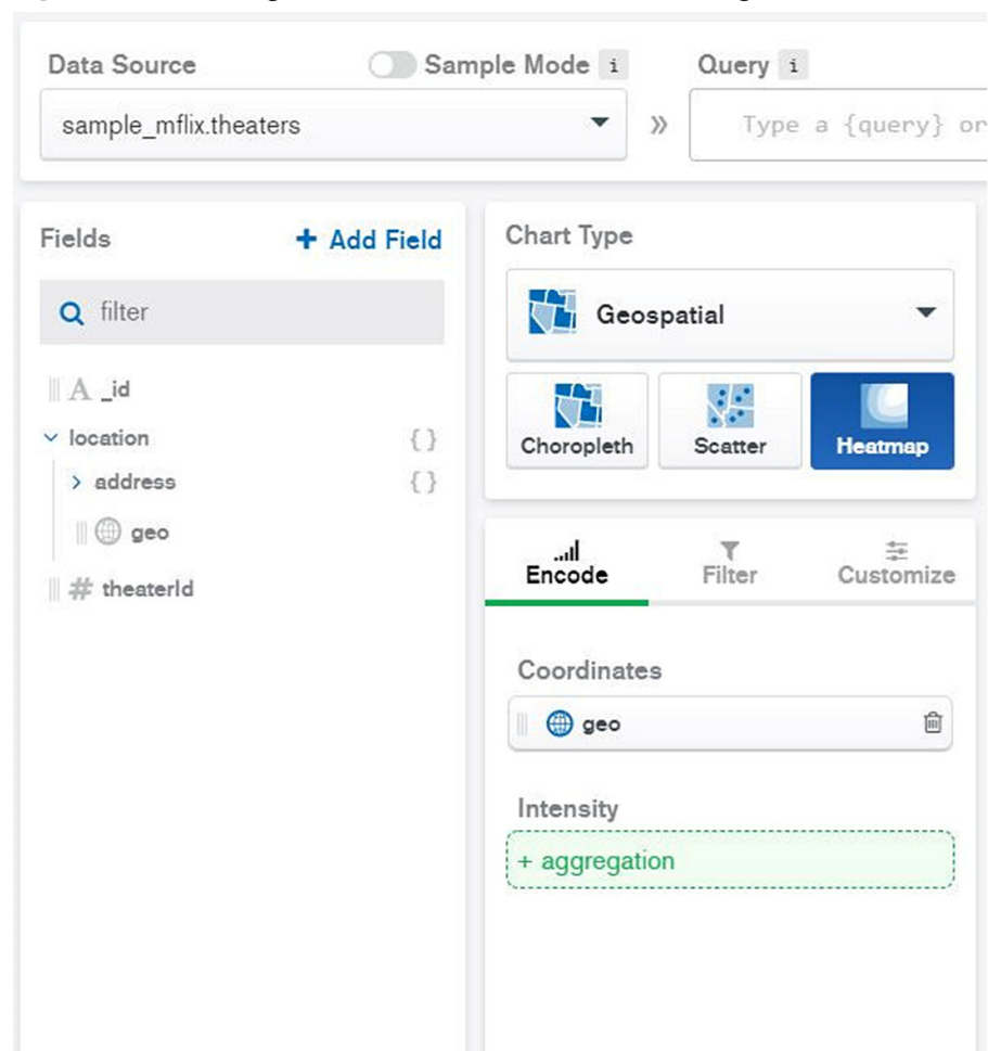
Figure 12.30: Dragging the geo field into the Coordinates encoding channel
