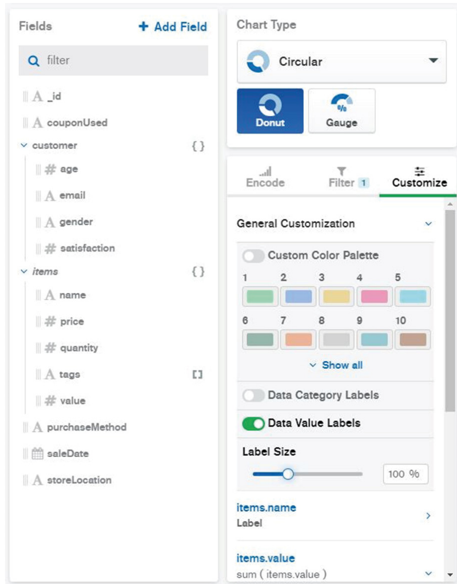
Figure 12.62: Customizing the data labels
