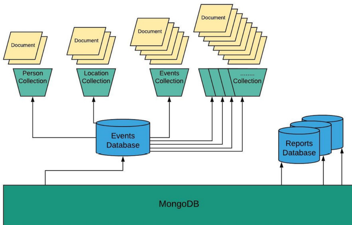
Figure 1.38: Pictorial representation of a MongoDB database
