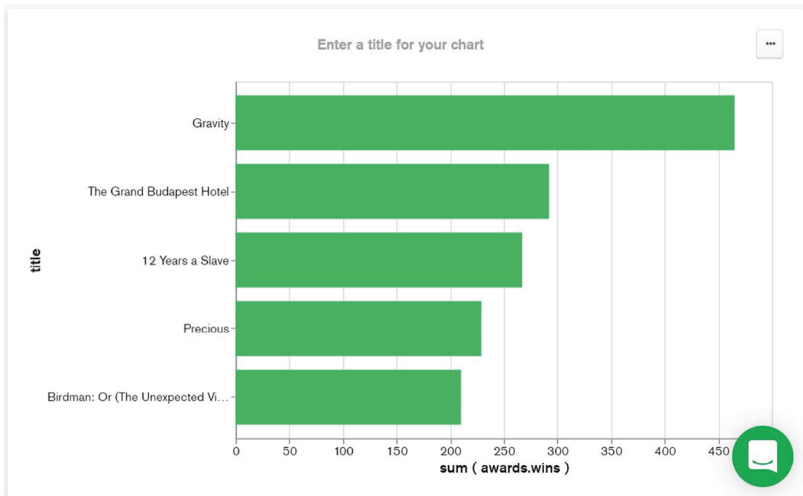
Figure 12.20: Top five movies sorted by the number of awards
