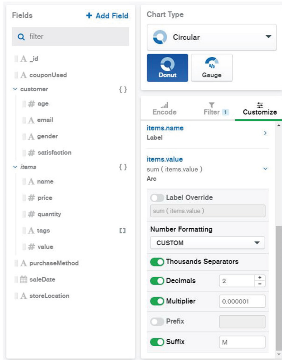
Figure 12.63: Customizing the chart formatting
