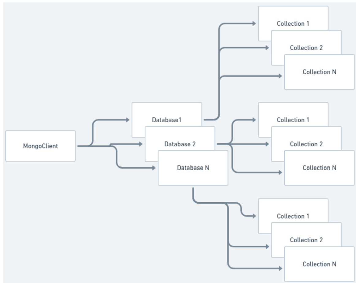
Figure 8.2: Driver entity relationships
