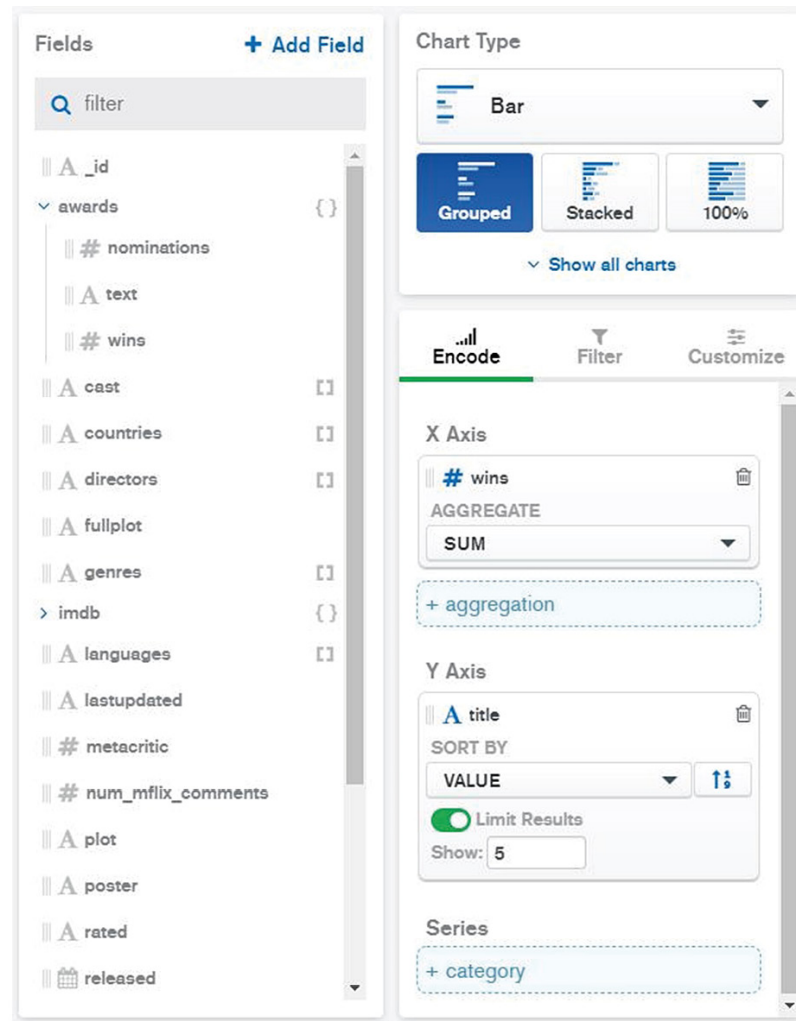
Figure 12.19: Adding the wins field to the X Axis
