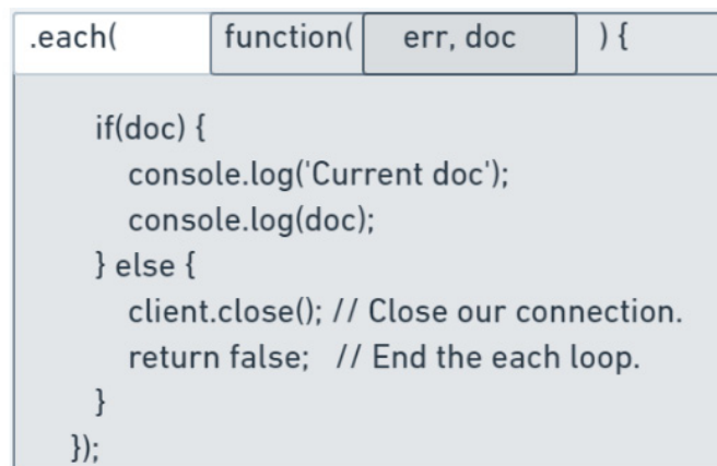
Figure 8.5: Breakdown of a MongoDB callback
