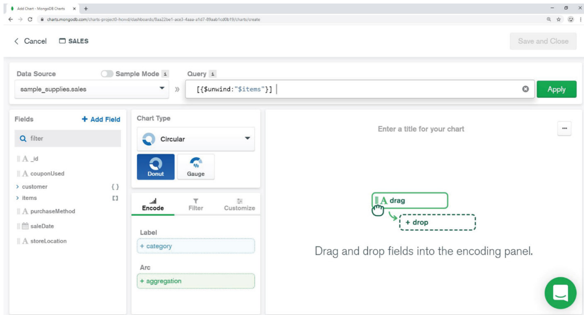
Figure 12.56: Writing the unwind function in the Query bar
