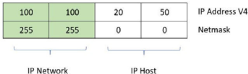
Figure 3.1: Diagrammatic representation of an IP address
