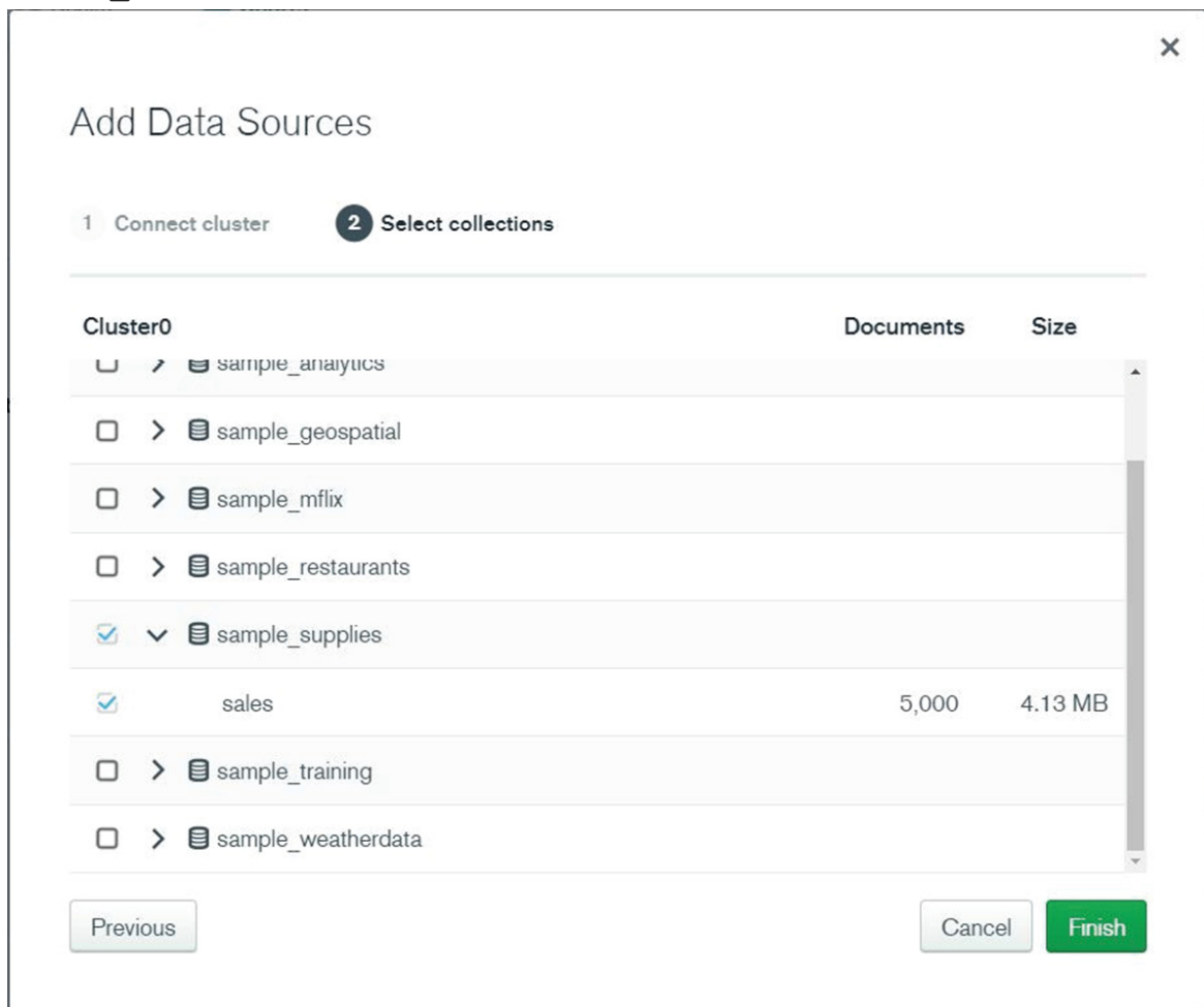
Figure 12.52: Creating a new sales data source
