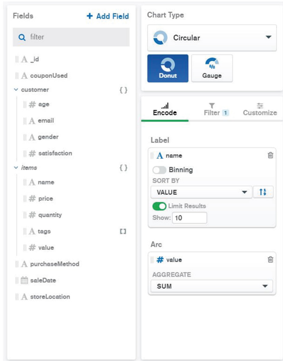
Figure 12.59: Dragging items.value into the Arc channel and choosing the SUM function
