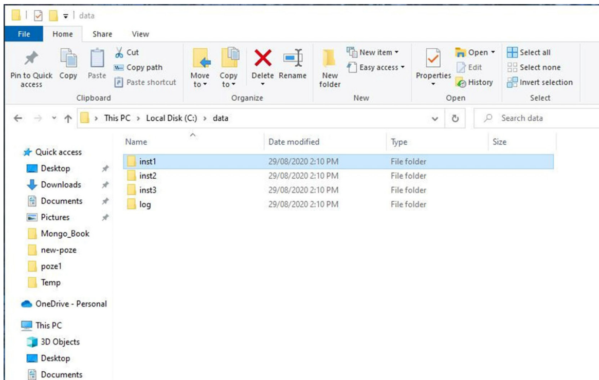
Figure 10.20: Directory structure
