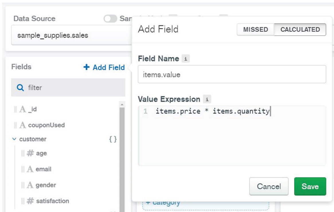
Figure 12.57: Adding the items.value field
