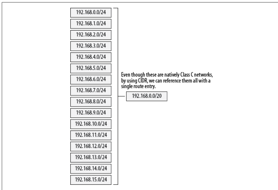
Figure 36-4. CIDR route aggregation
