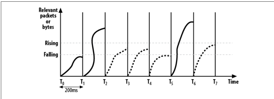
Figure 19-3. Rising and falling thresholds
