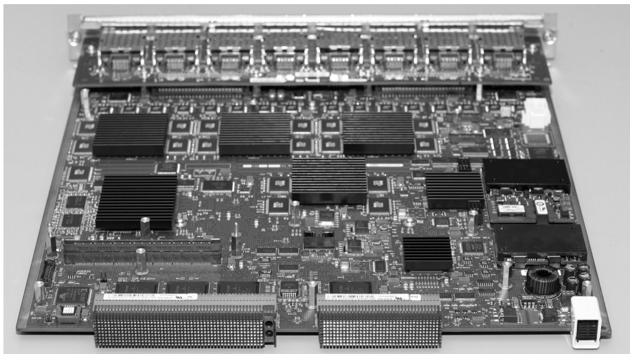
Figure 17-6. Fabric-enabled blade connectors
