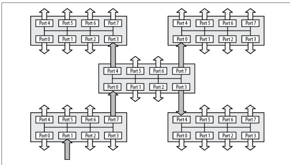
Figure 2-5. Hub-based network
