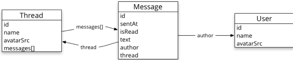
Redux Chat Models
