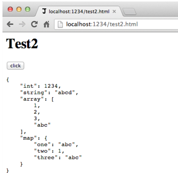
Figure 7—JSON term sent from Erlang
