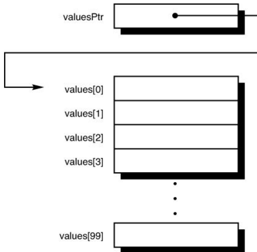
Figure 10.9 Pointer to an array element.
