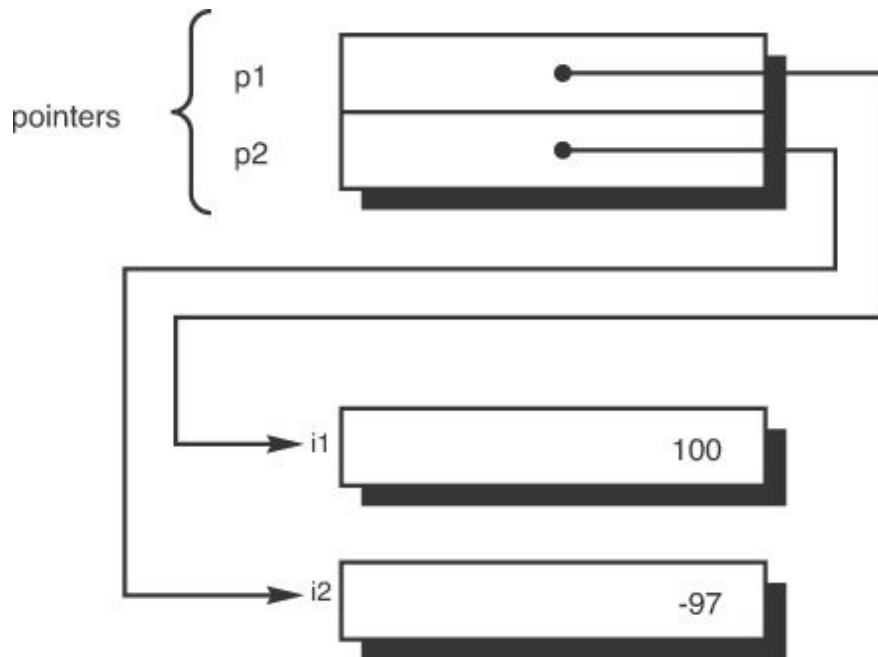
Figure 10.3 Structure containing pointers.
