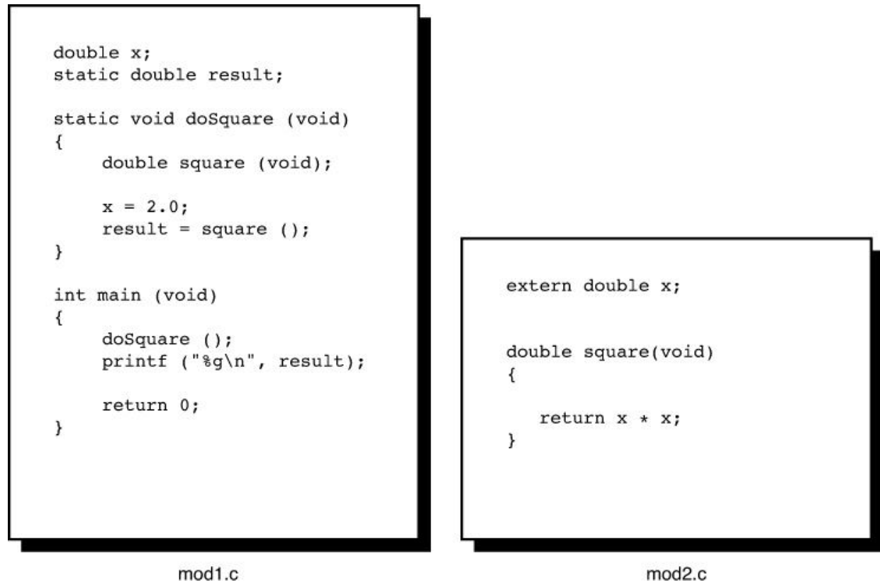
Figure 14.1 Communication between modules.
