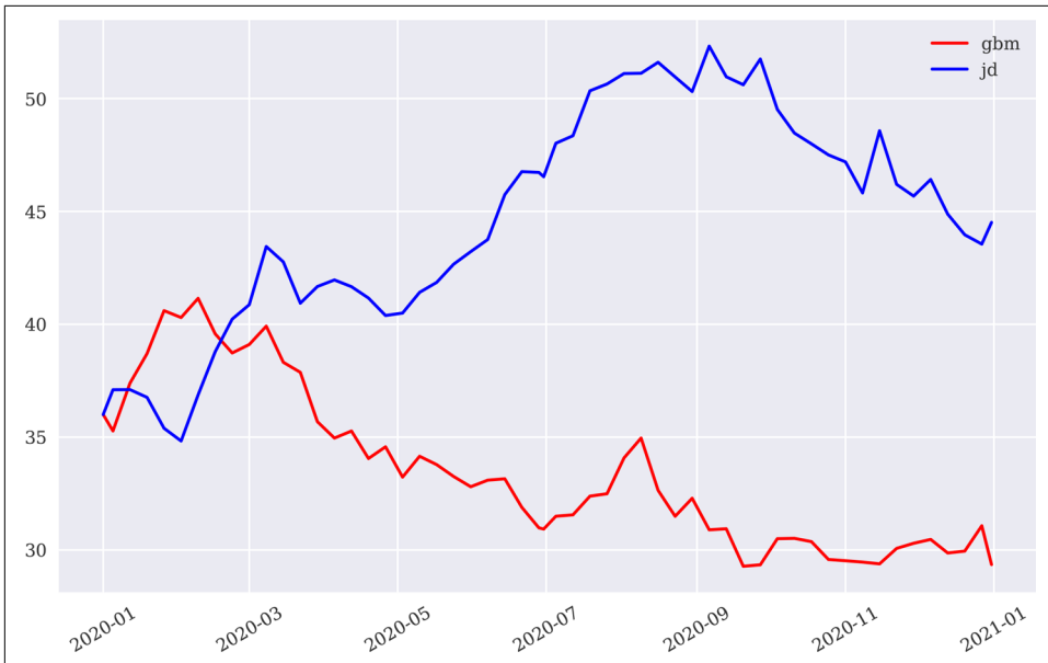
Figure 20-1. Noncorrelated risk factors (two sample paths)
