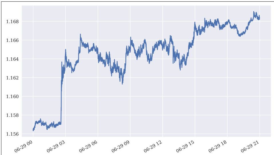
Figure 8-14. Tick data for EUR/USD exchange rate
