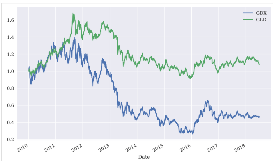
Figure 13-19. Normalized prices for GLD and GDX over time
