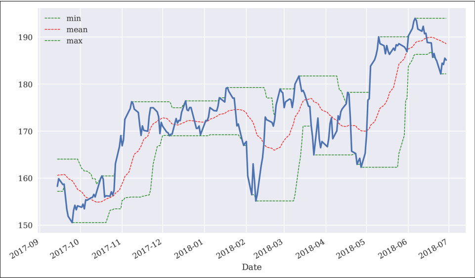
Figure 8-5. Rolling statistics for minimum, mean, maximum values
