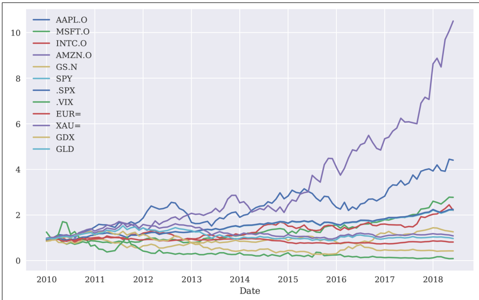
Figure 8-4. Resampled cumulative log returns over time (monthly)
