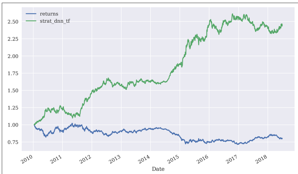
Figure 15-19. Performance of EUR/USD and DNN-based trading strategy (TensorFlow, in-sample)
