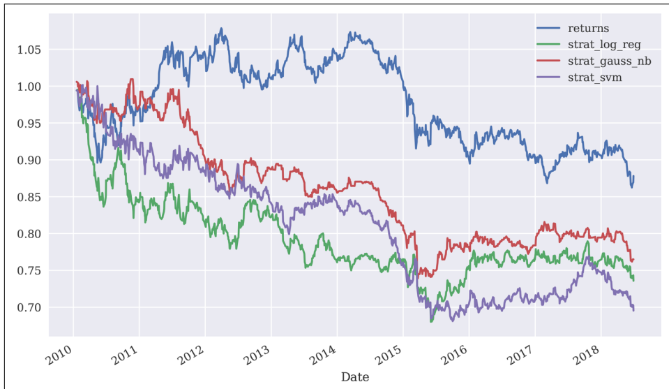
Figure 15-16. Performance of EUR/USD and classification-based trading strategies (randomized train-test split)
