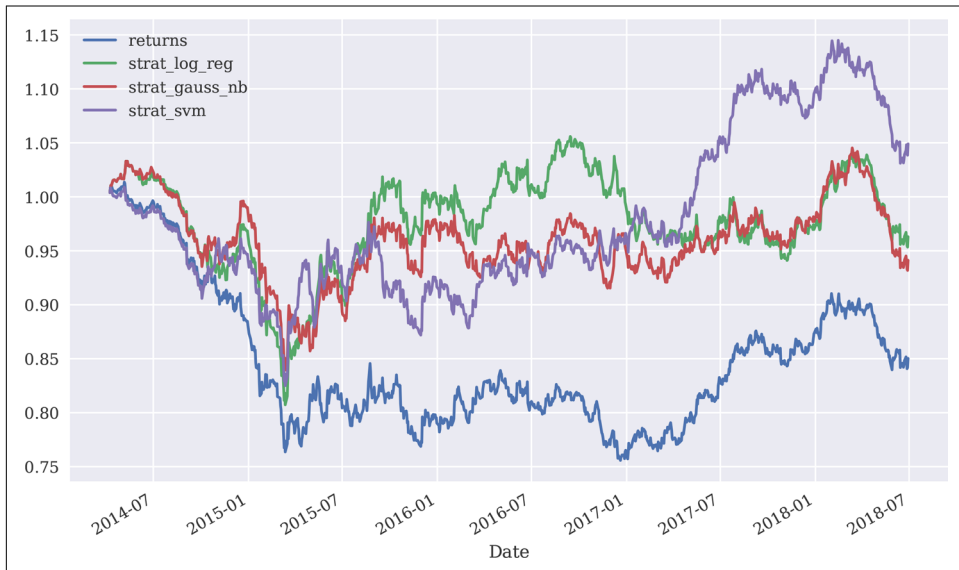
Figure 15-15. Performance of EUR/USD and classification-based trading strategies (sequential train-test split)
