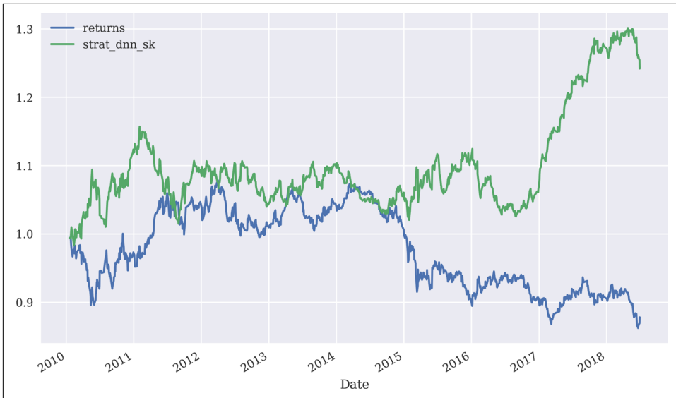
Figure 15-18. Performance of EUR/USD and DNN-based trading strategy (scikit-learn, randomized train-test split)
