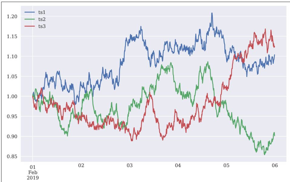
Figure 9-8. A specific time interval of the financial time series (normalized)
