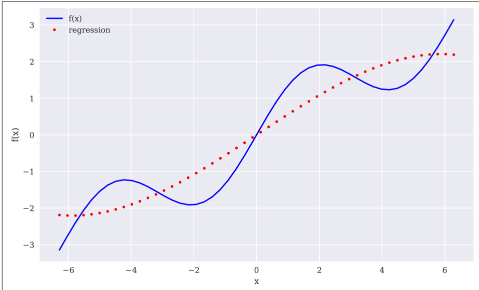
Figure 11-5. Regression with individual basis functions
