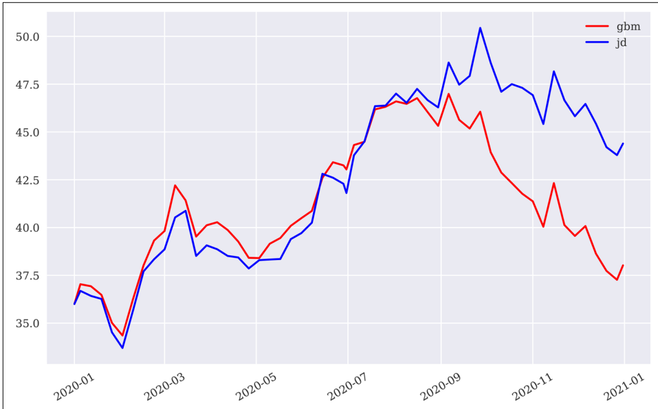
Figure 20-2. Correlated risk factors (two sample paths)
