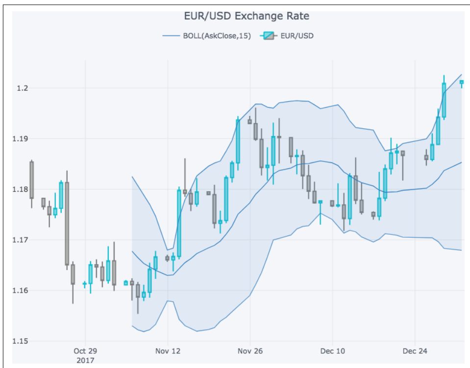
Figure 7-26. OHLC plot of EUR/USD data with Bollinger band
