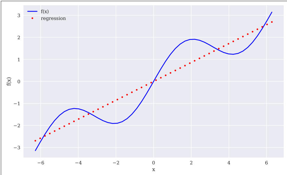
Figure 11-2. Linear regression
