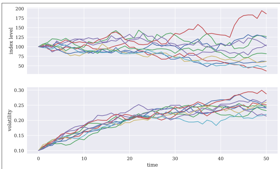
Figure 12-12. Dynamically simulated stochastic volatility process paths
