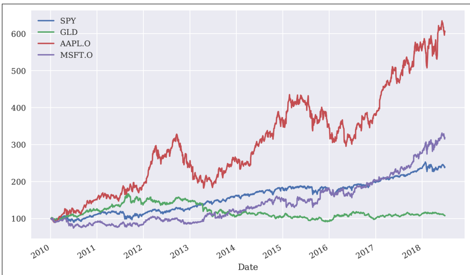
Figure 13-7. Normalized prices of financial instruments over time
