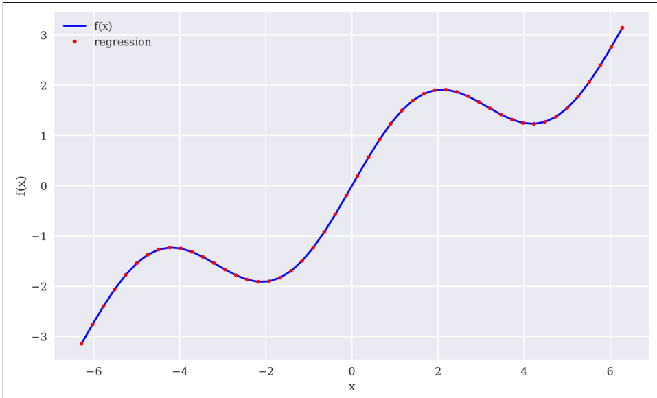
Figure 11-6. Regression with the sine basis function
