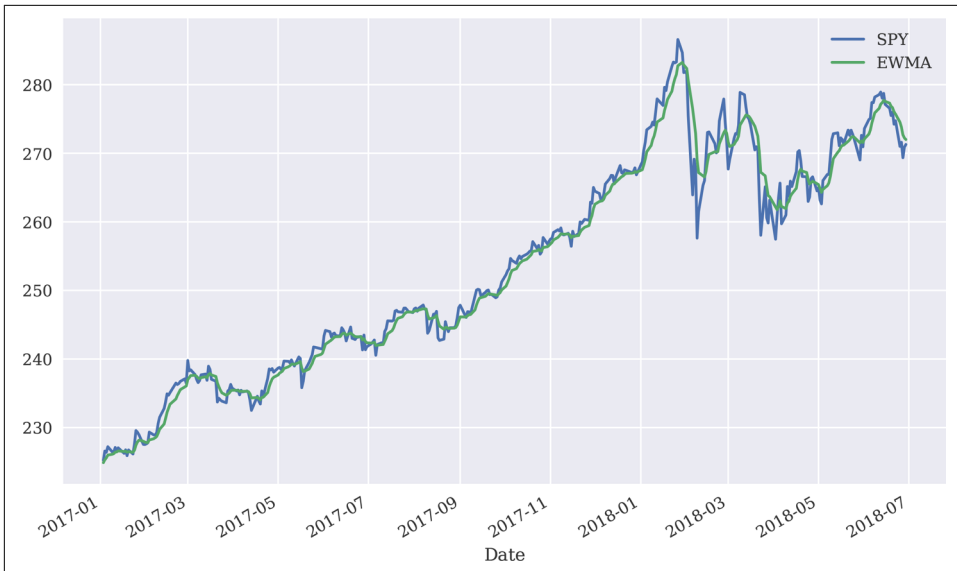
Figure 10-3. Financial time series with EWMA
